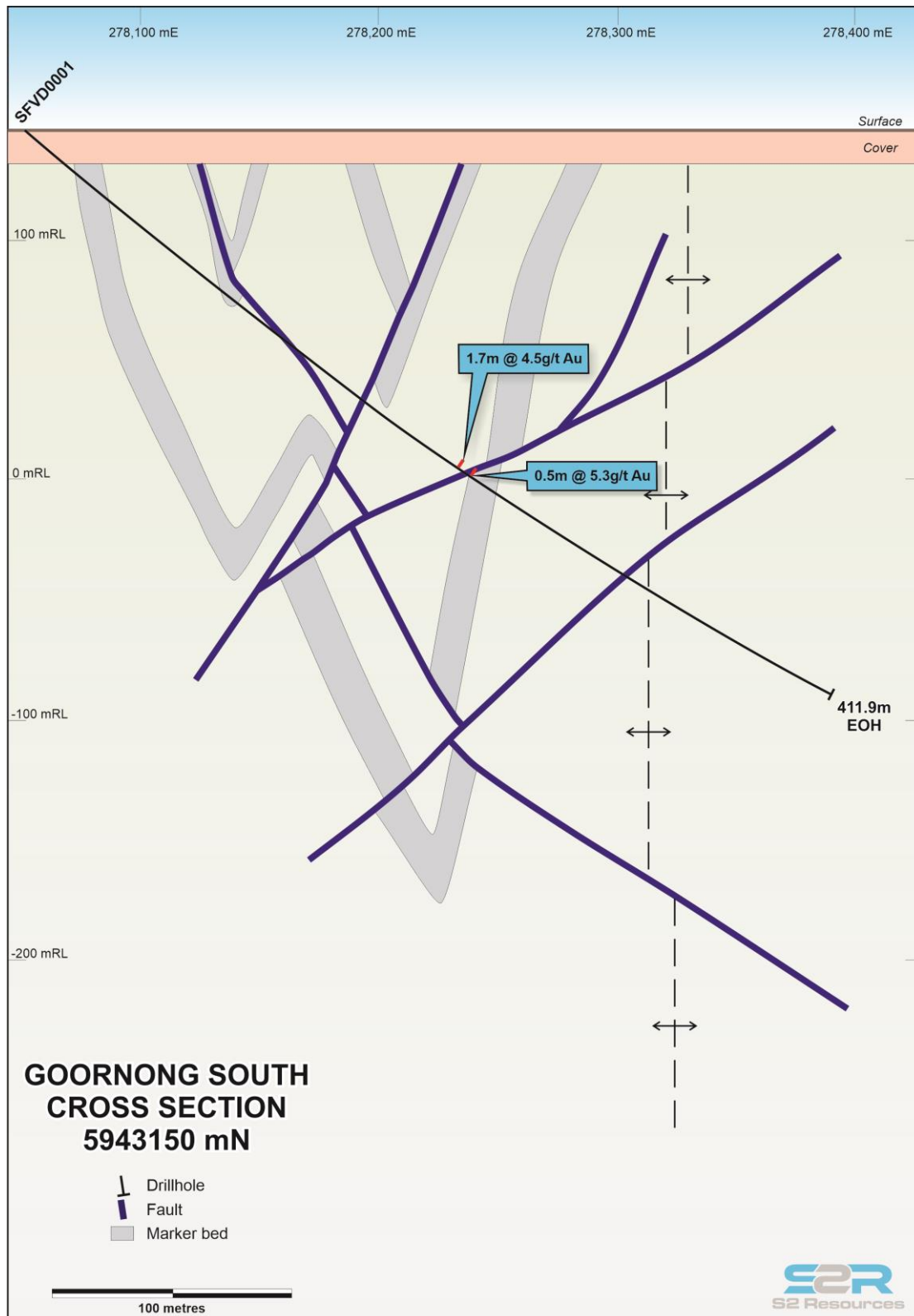
Figure 2. Cross section of the Goornong South area showing drill hole SFVD0001 that tested the favourable anticlinal hinge zone south of the oxide gold mineralisation.
