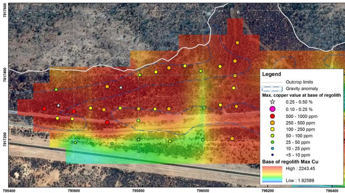
Figure 4 – Copper at base of regolith at the Guchab South target, from the results of the RC drilling program.
