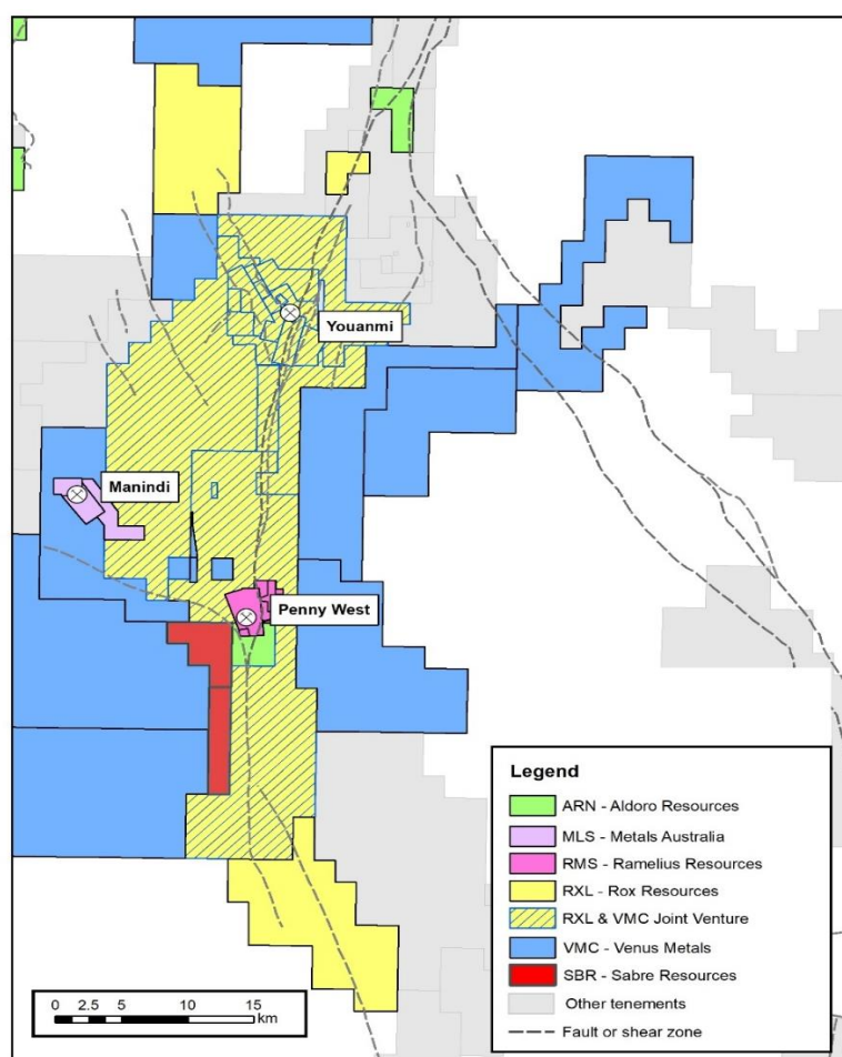
Figure 3: ASX listed companies active in the Youanmi area showing main structural trends
