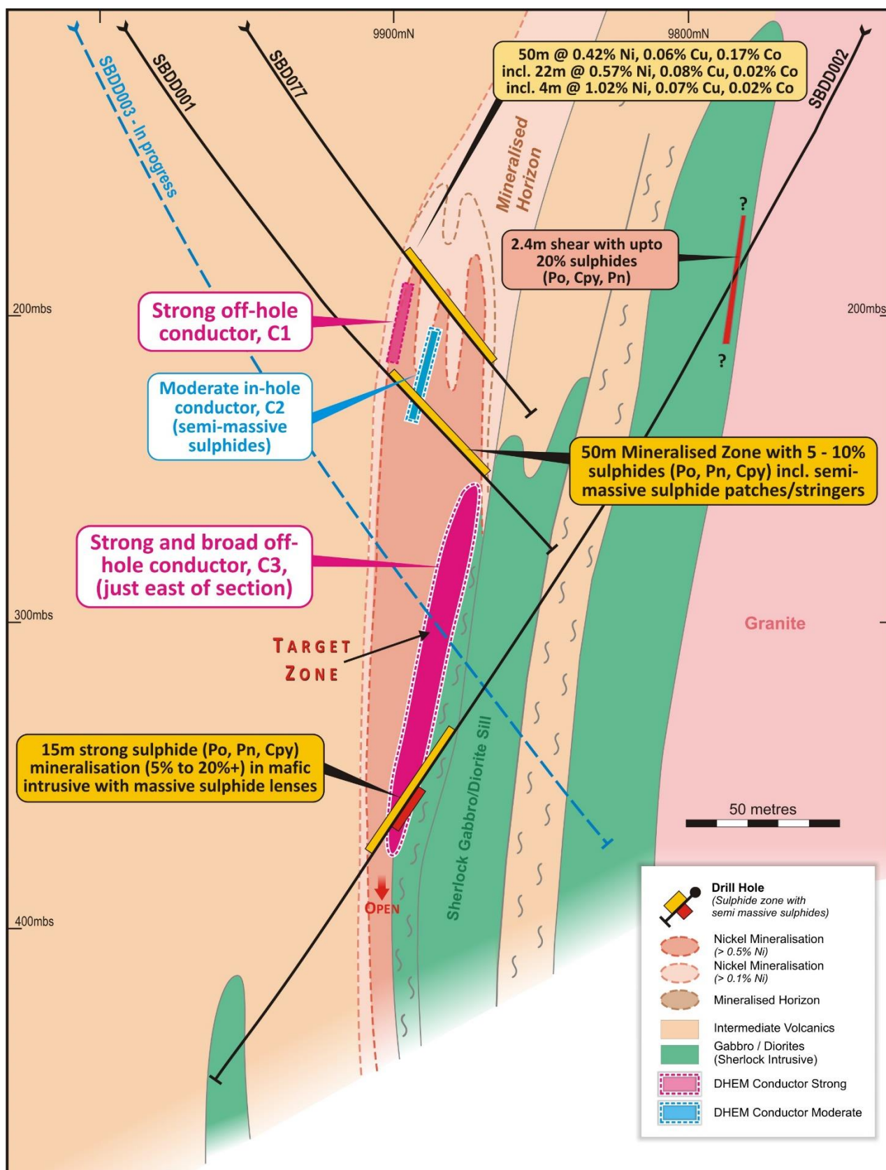
Figure 1: Sherlock Bay cross section 19,600mE with DHEM conductors, Target Zone and drilling completed.
