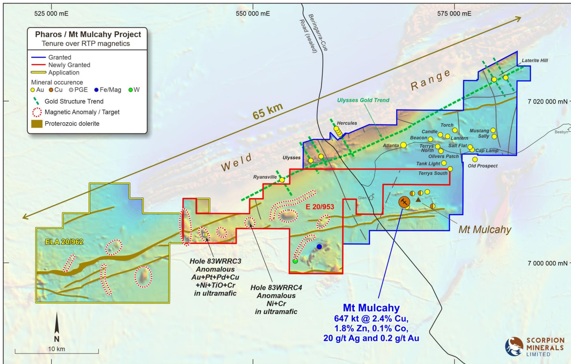
Figure 3 – Location of Ultramafic Targets on E20/953 and historic CRA Pty Ltd RC drilling overlain on regional magnetics
