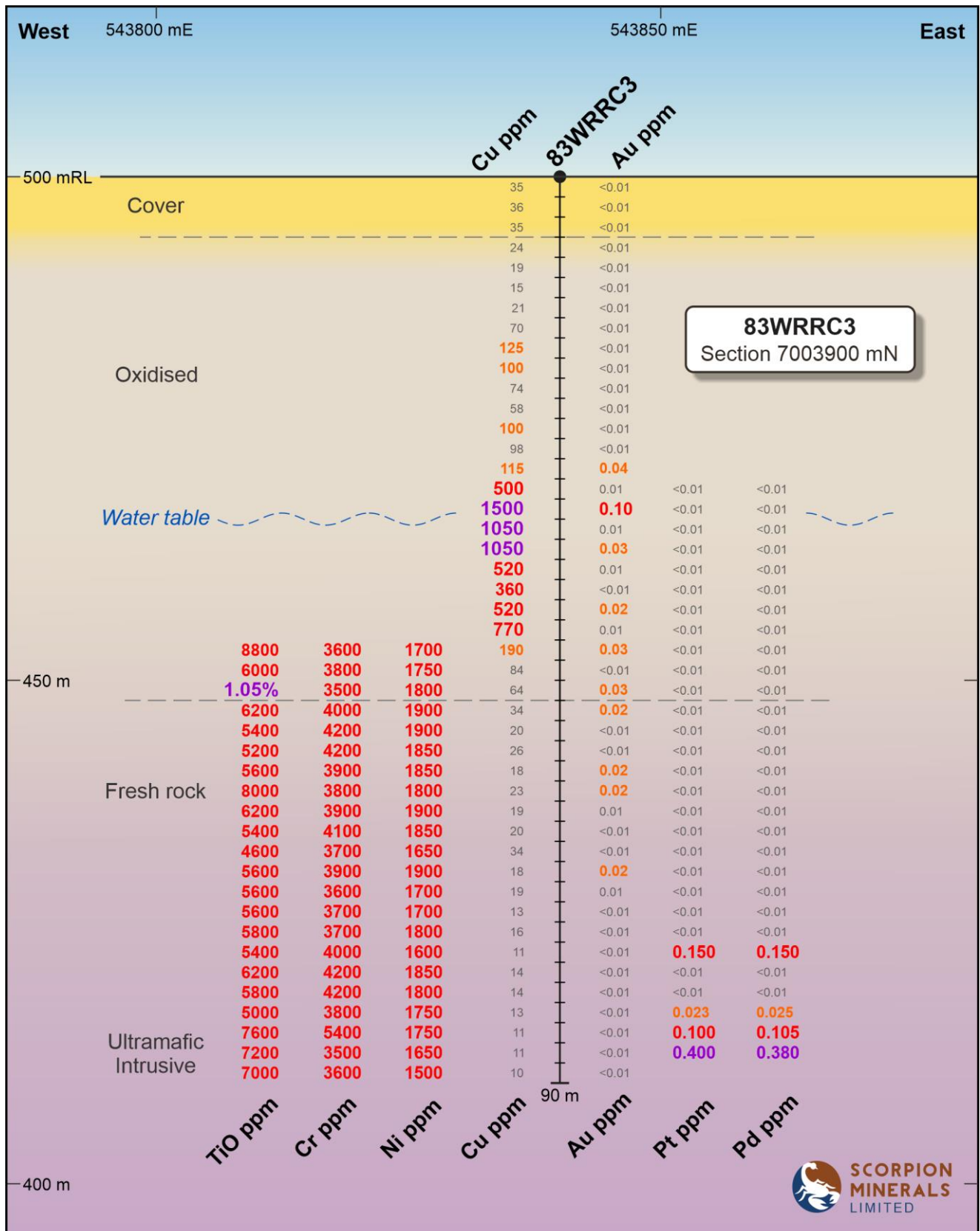
Figure 4 – Cross Section of 83WRRRC3 showing anomalous Pd/Pt, Ni, CU, Au, Cr and Ti
