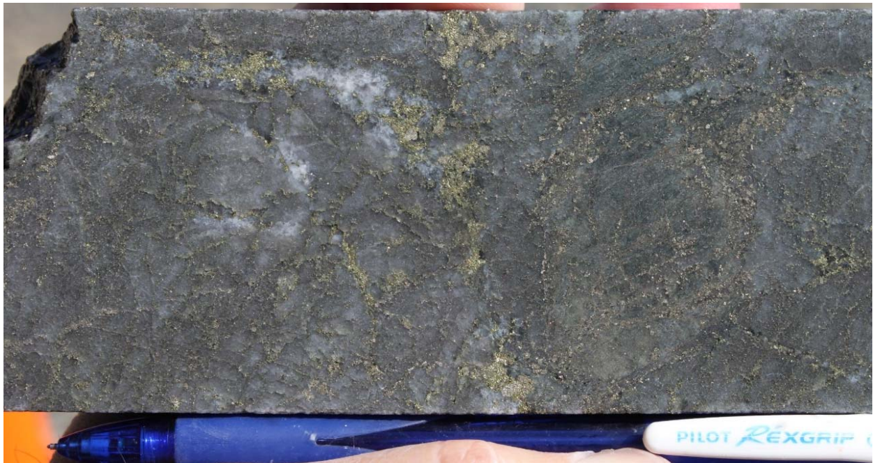
Figure 14: Core photo at 347m down-hole showing the mineralisation style intersected in TMMRD006
