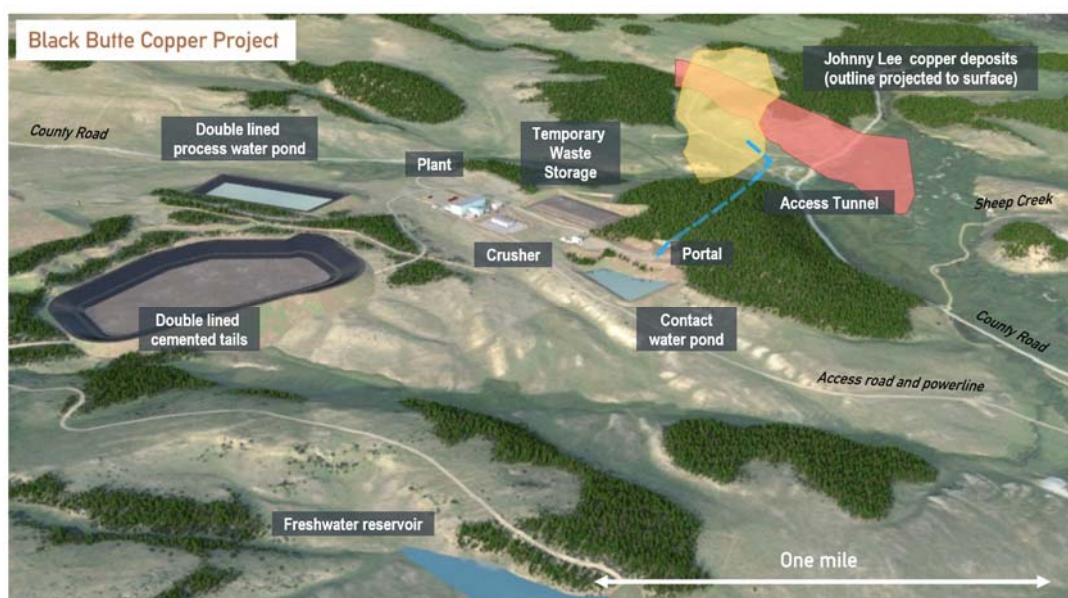
Figure 5: Black Butte Copper Project – Proposed Site Layout
