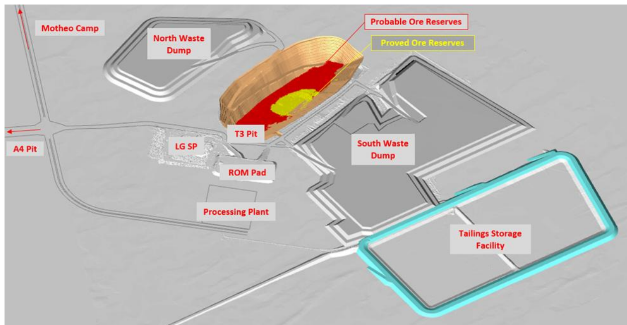
Figure 12: T3 Copper Project – Site Layout
