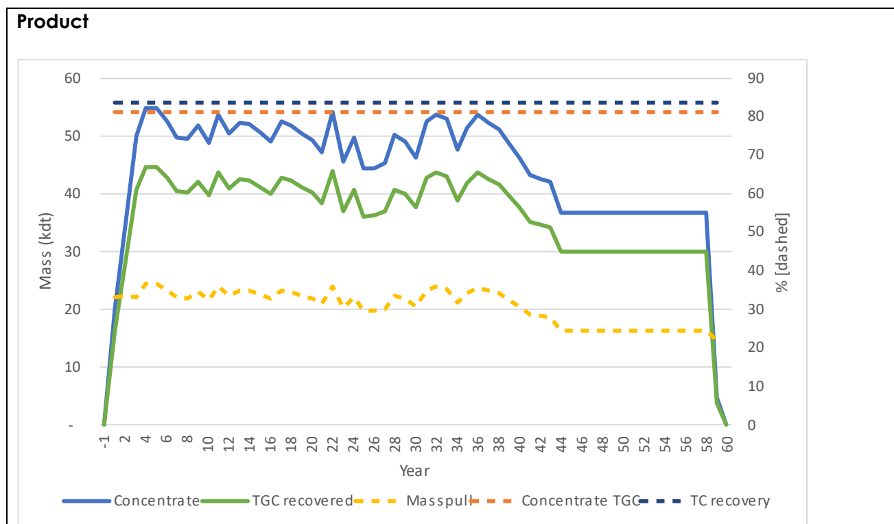
Figure 9 - Mining production schedule summary
