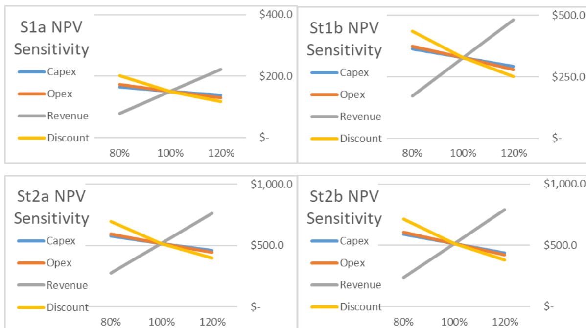
Figure 24 - Sensitivity Analysis
