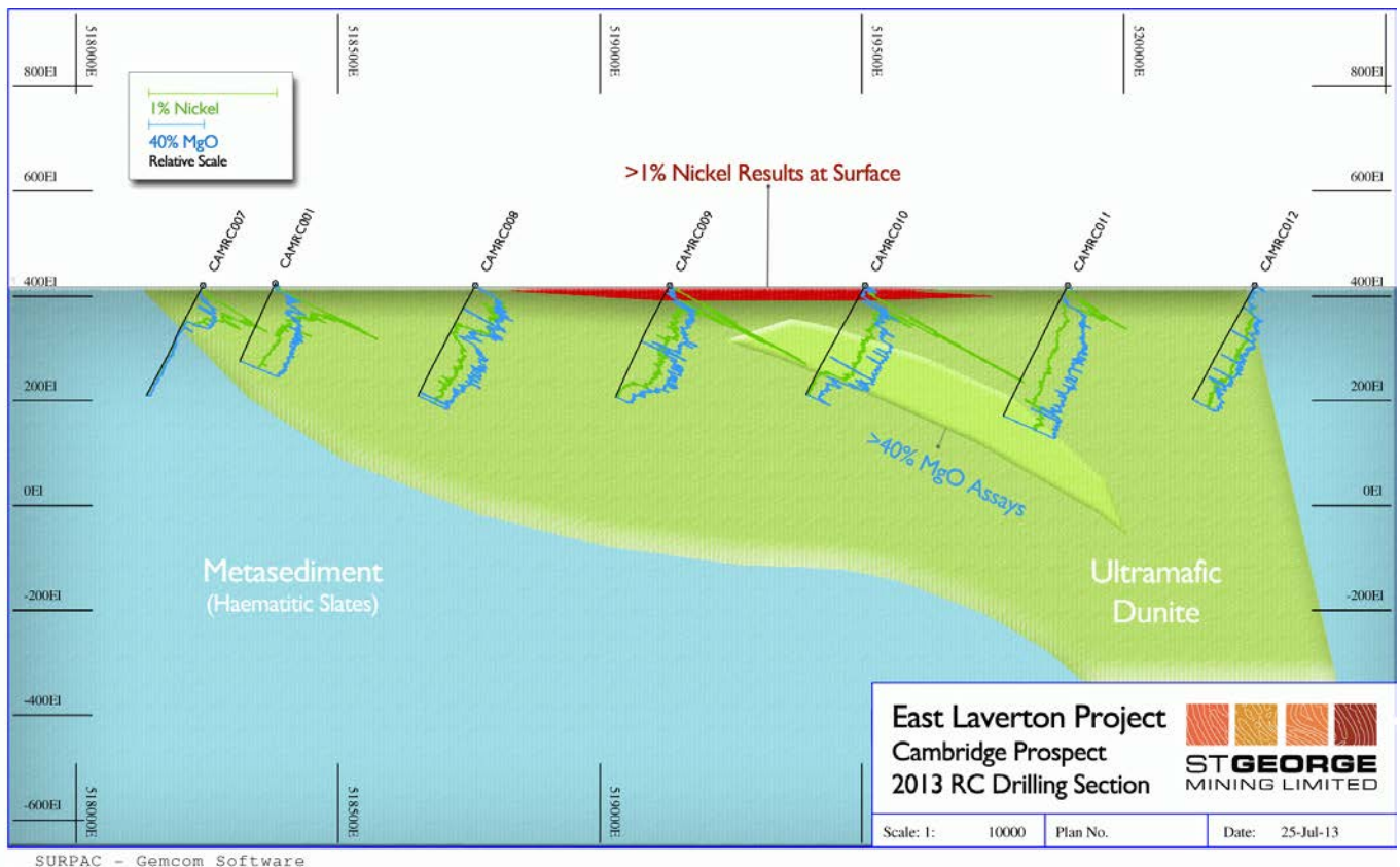
Figure 2- Drill section across the Cambridge ultramafic body shows the highest Ni values (green lines) and MgO values (blue lines) in the central zone. The MgO content of the ultramafic increases with depth and dips to the east. The deepest contact with this easterly dipping high-MgO zone is made in CAMRC-011, which intersects 42 m @ 0.26%Ni and 40.1 % MgO at the base of the hole, and appears to have encountered the top of an olivine adcumulate zone.
