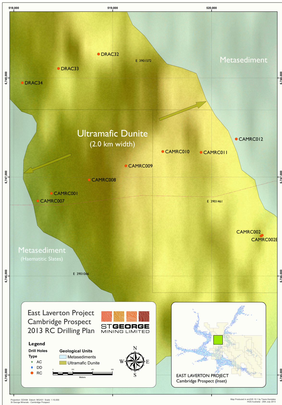
Figure 1 – 2013 drill hole locations across the Cambridge ultramafic body. CAMRC001 and 002 were drilled by the Company in 2012. DRAC32, 33 and 34 were completed in 2012 as part of Project Dragon.
