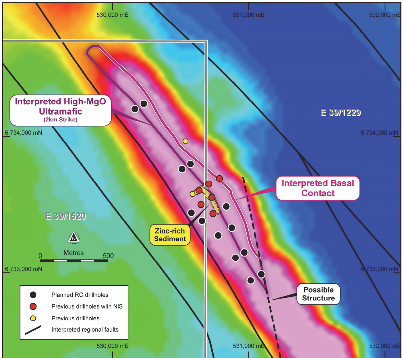
Figure 1 – interpreted ultramafic at Windsor against TMI magnetics showing the small area tested to date and highlighting the substantial exploration upside. The eastern basal contact will be tested by the 4,000m RC drilling programme currently underway. All holes will be drilled to the northeast.
