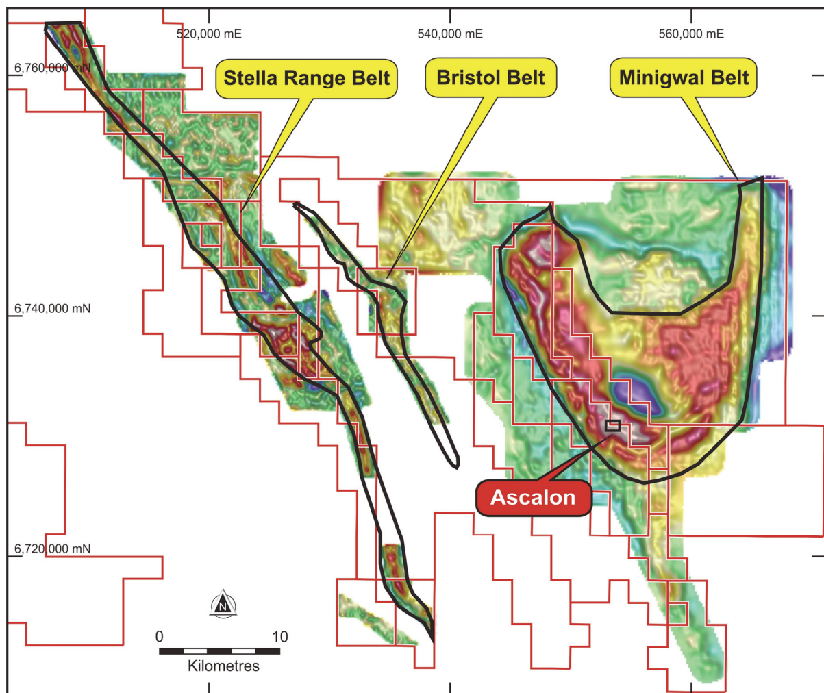
Figure 2 – the East Laverton tenements with 1VD Bouguer gravity data. The strongest gravity features (red colour) are present in the Minigwal belt where Ascalon is located.
