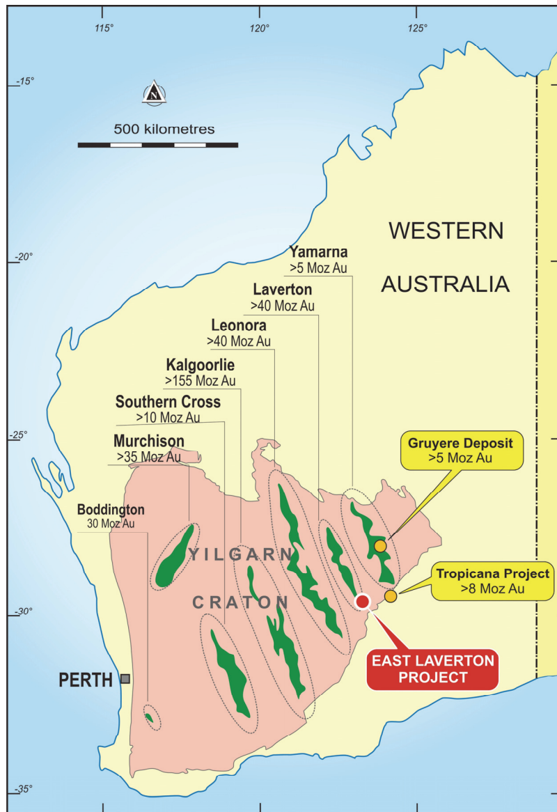
Figure 1 – the main gold-bearing greenstone belts of the Yilgarn Craton. The East Laverton Project is within the North Eastern Goldfields, along with Tropicana and Gruyere.
