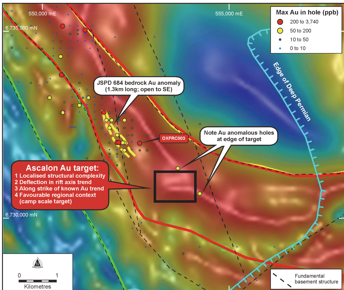
Figure 1 – the Ascalon target shown against gravity data. OXFRC003 has confirmed that the copper-gold anomalism continues along strike towards Ascalon and at significant widths.
