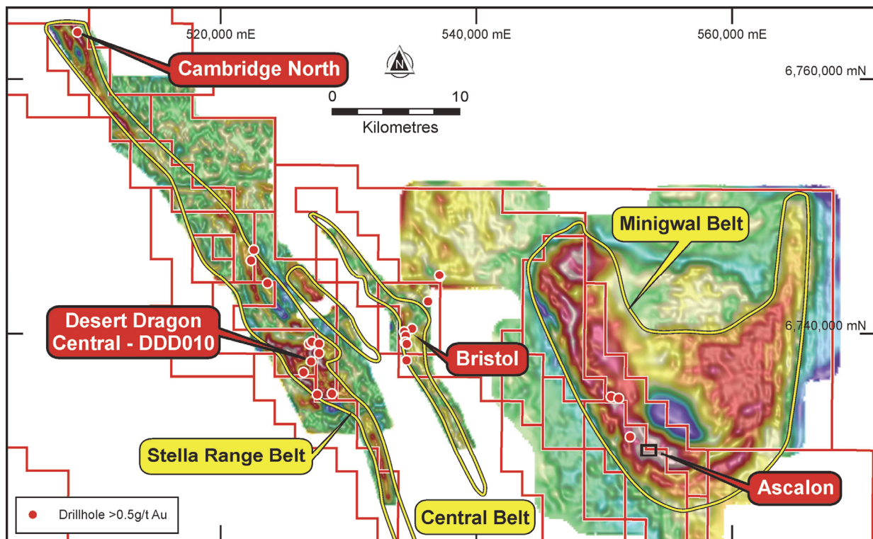
Figure 2 – the East Laverton tenements against FVD Bouguer gravity data. Ascalon is located in the thickest part of the Minigwal belt. Gold targets at Bristol, DDD010 and Cambridge North are also scheduled to be tested in the upcoming gold drilling campaign.
