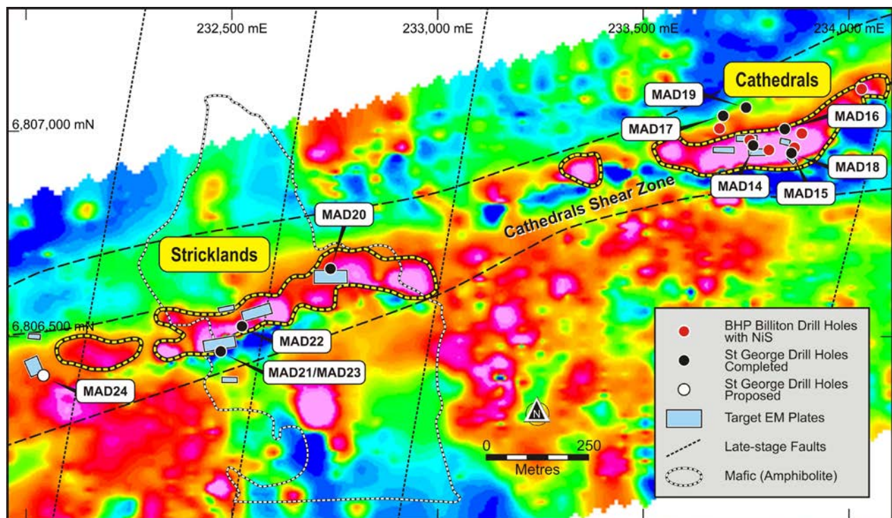
Figure 2 – a plan view of the Cathedrals and Stricklands Prospects over TMI magnetics showing the EM conductors at Stricklands and the drill hole collar locations in the current programme.
