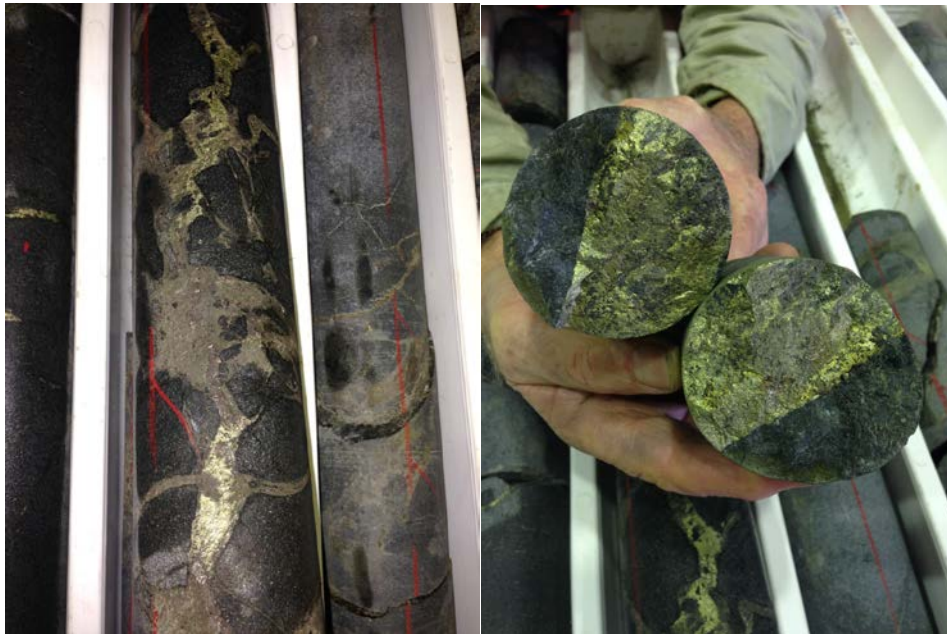
Figure 2 – on left : drill core from MAD22 at 51m downhole showing brecciated massive sulphides and veinlets, indicating structural remobilisation from a massive sulphide source. On right : drill core from MAD22 with massive chalcopyrite (yellow-green) in contact with ultramafic (dark grey). Assays for this interval (52.4-52.63m) returned 13.1%Cu and 43g/tAg.
