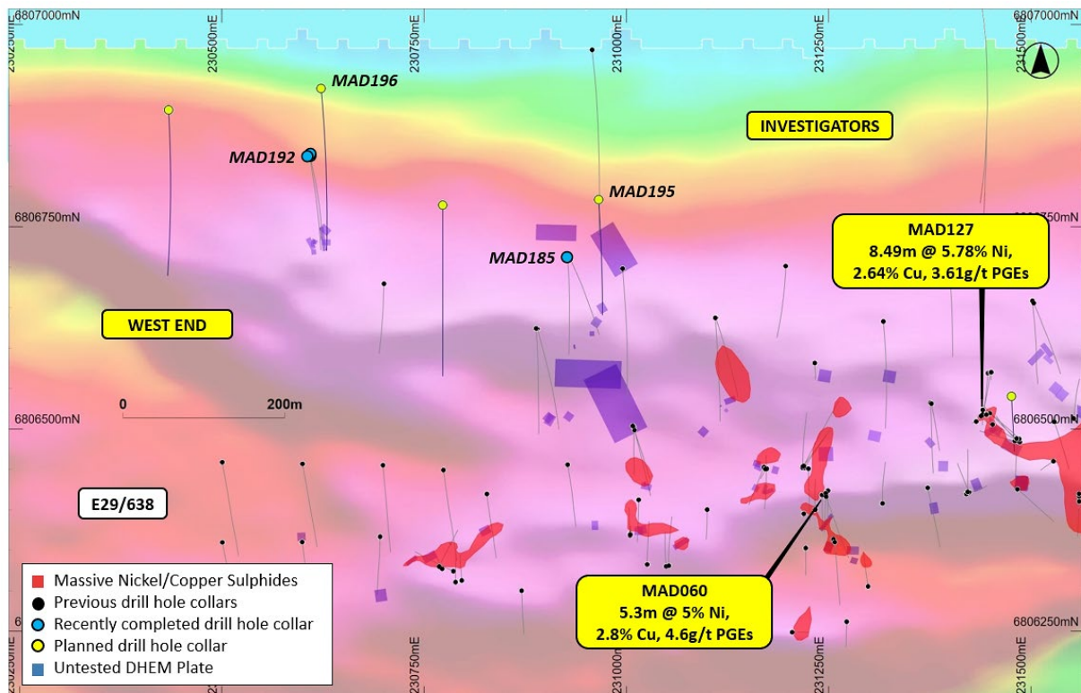
Figure 2 (below) – plan view map (against MMR data) of the West End and western Investigators Prospect areas showing the location of the drill holes underway (MAD195 and MAD196), the new EM plates modelled from the latest DHEM surveys and some of the high-grade intersections at Investigators.
