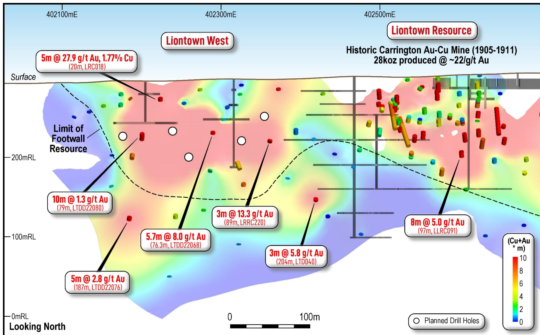
Figure 3: Long section (20m thick) of the Au-Cu rich footwall horizon at Lontown West, coloured by thickness. Key historic intercepts, historic workings including the Carrington Au-Cu Mine and planned infill RC holes (white dots) are displayed.
