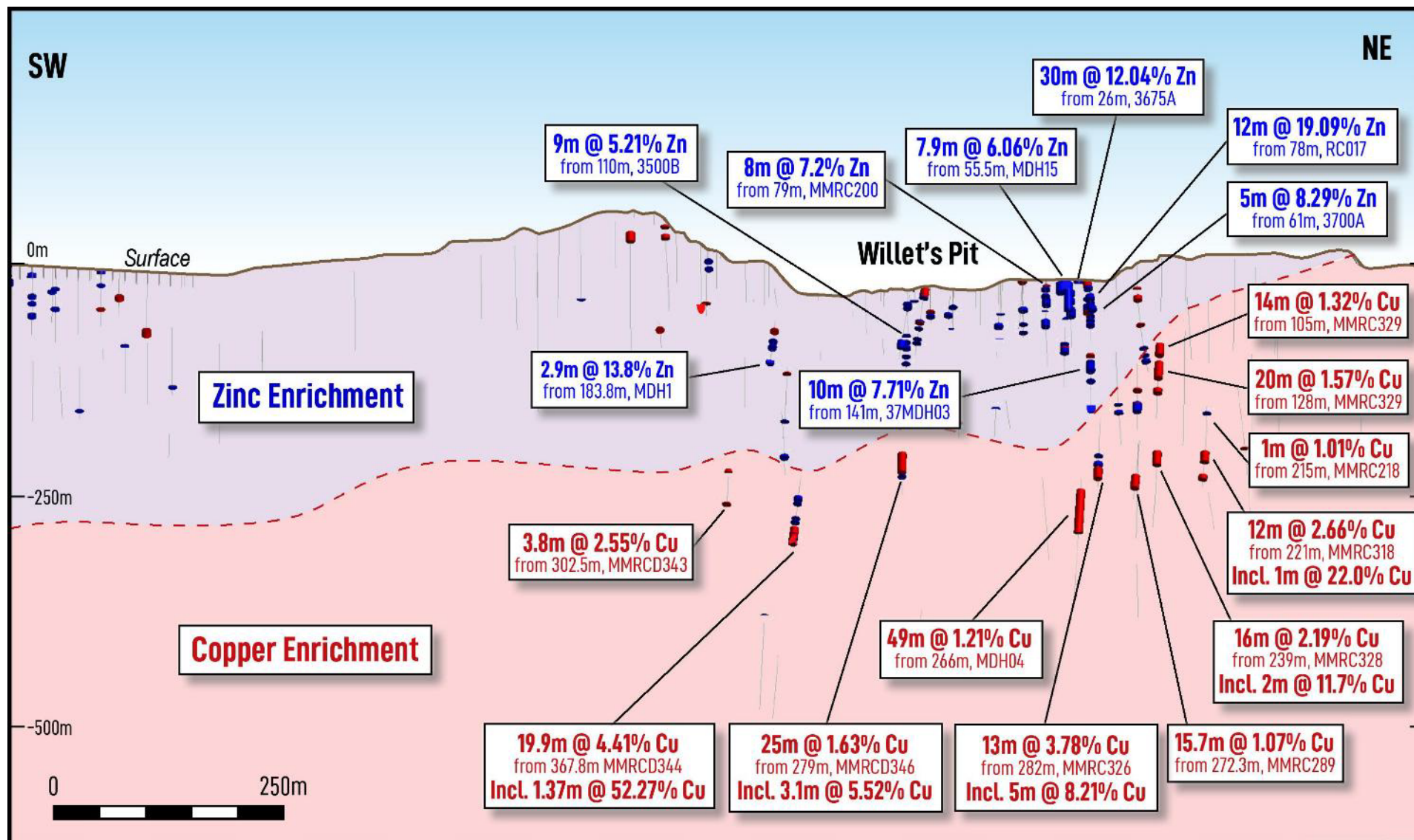
Figure 6. Mt Moss long section (SW to NE on previous page – Figure 5) looking north showing zonation in base metal mineralisation, with zinc dominant at shallow depths appearing to grade into copper rich mineralisation at depth.
