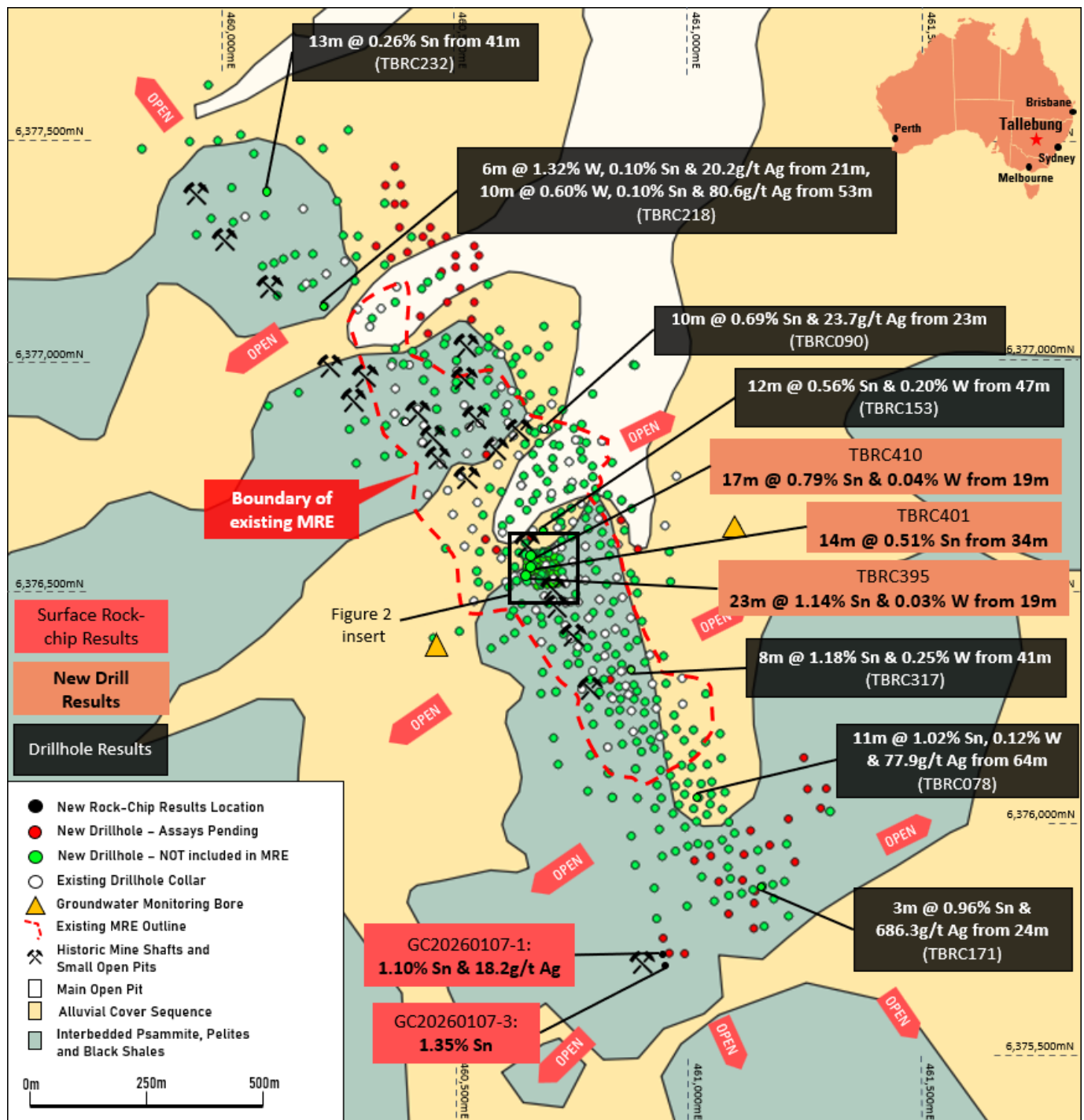
Figure 1: Plan showing the location of new drilling results. Drill-hole collars, previously reported highlight drill intercepts and the limits of the existing Talibung MRE are shown over surface geology.
