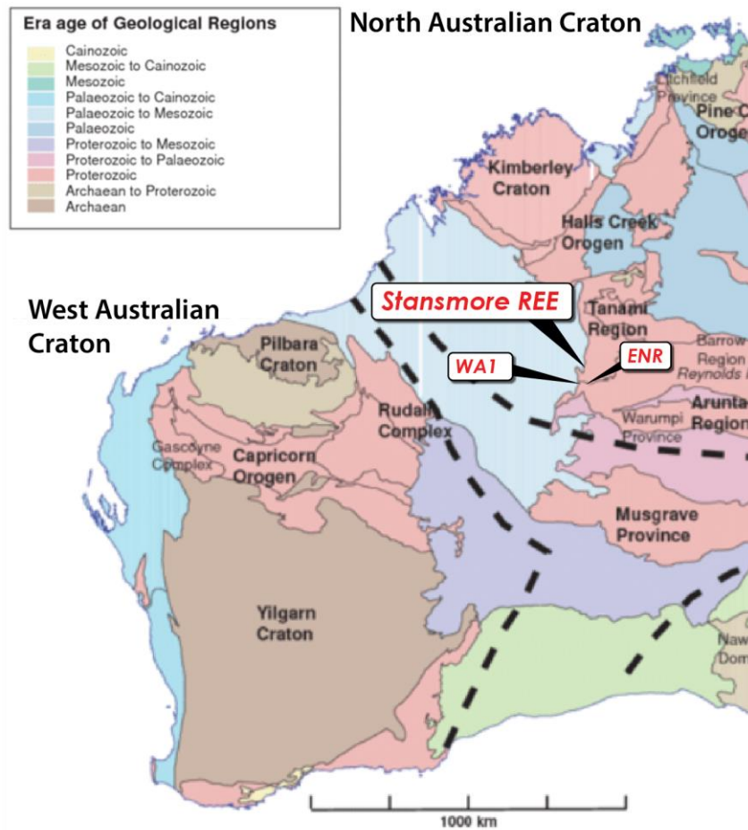
Figure 2. Stansmore REE Carbonatite – IOCG Project (Map overlay, Geodynamic and metallogenic evolution of Proterozoic Australia) 3 .
