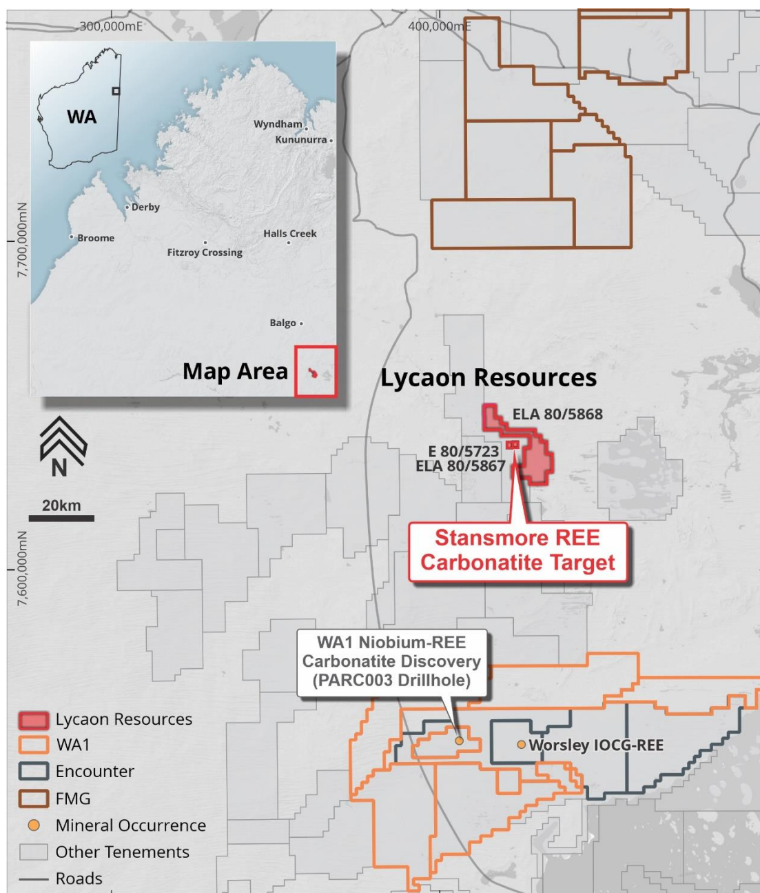
Figure 1. Stansmore REE Carbonatite – IOCG Project Location Map.
