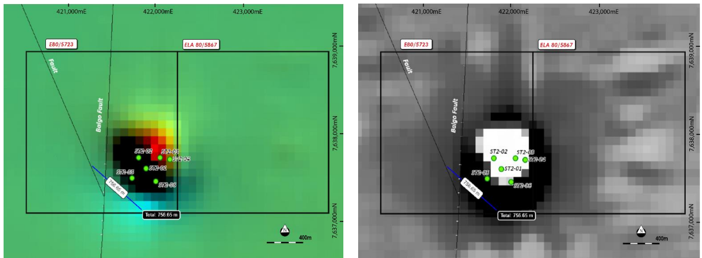
Figure 6. Drilling at Stansmore (refer Appendix 1) overlain on magnetics TMI and 1VD imagery. Source DMIRS Geoview
