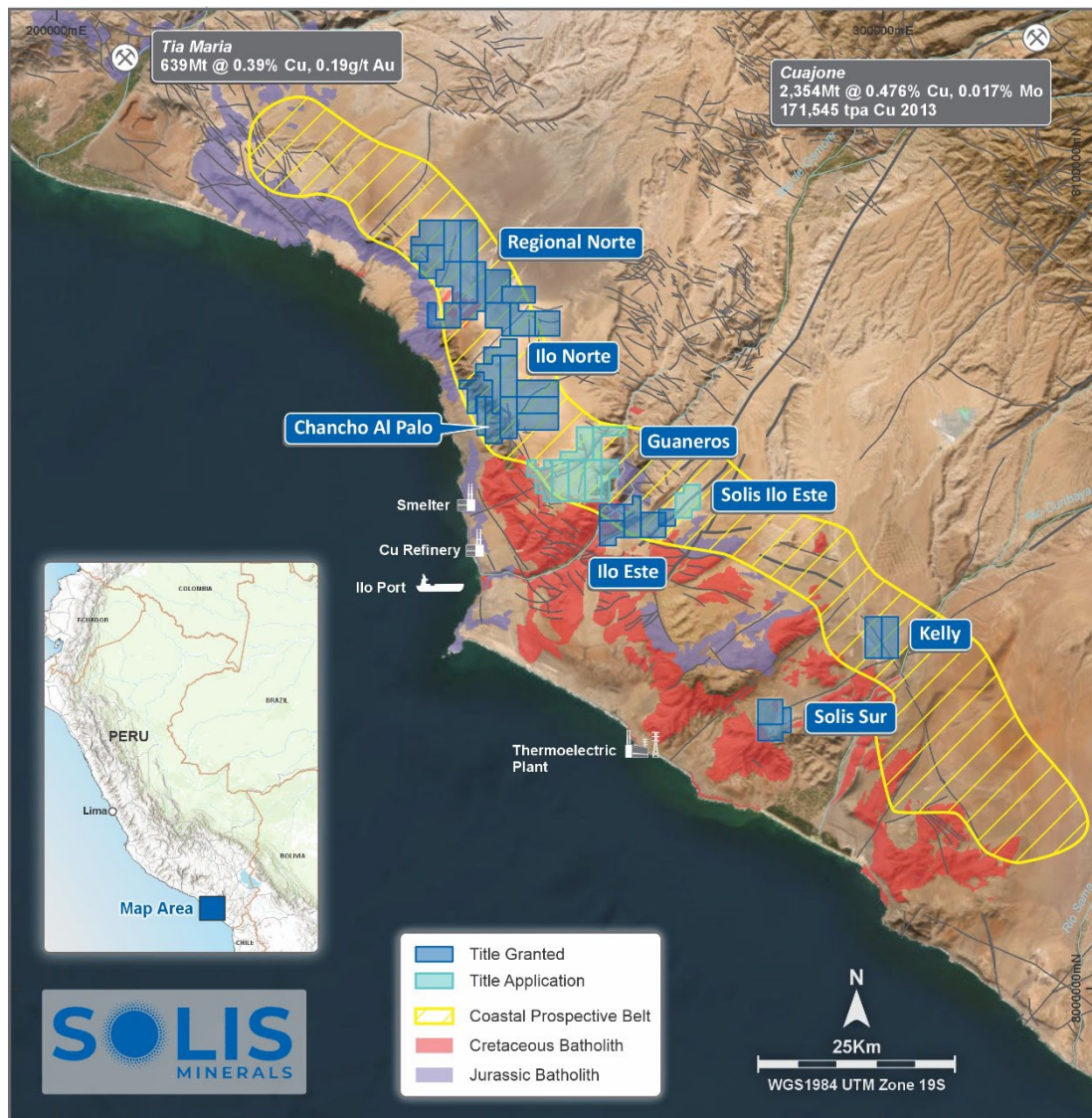
Figure 2: Solis tenements in the prospective coastal belt of Peru with existing deposits and regional geology.
