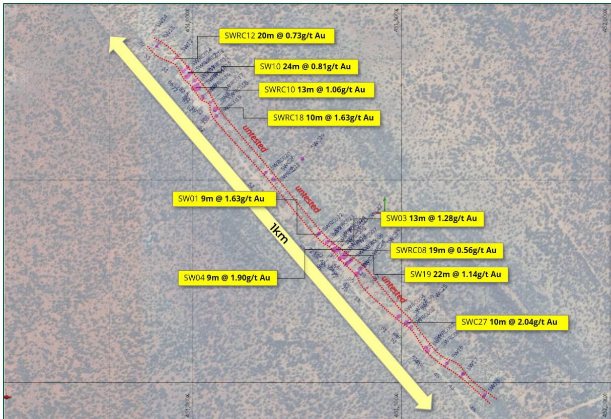
Figure 3. Statesman Well plan view showing all drillhole traces, significant results and untested segments of the mineralised surface.
