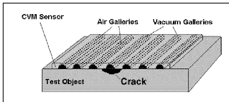
Figure 1. Measuring principle of the CVM Technology
