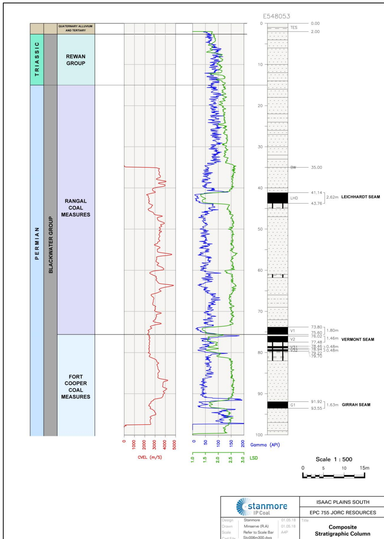
Figure 2: Isaac South EPC 755 – Typical Stratigraphic Column
