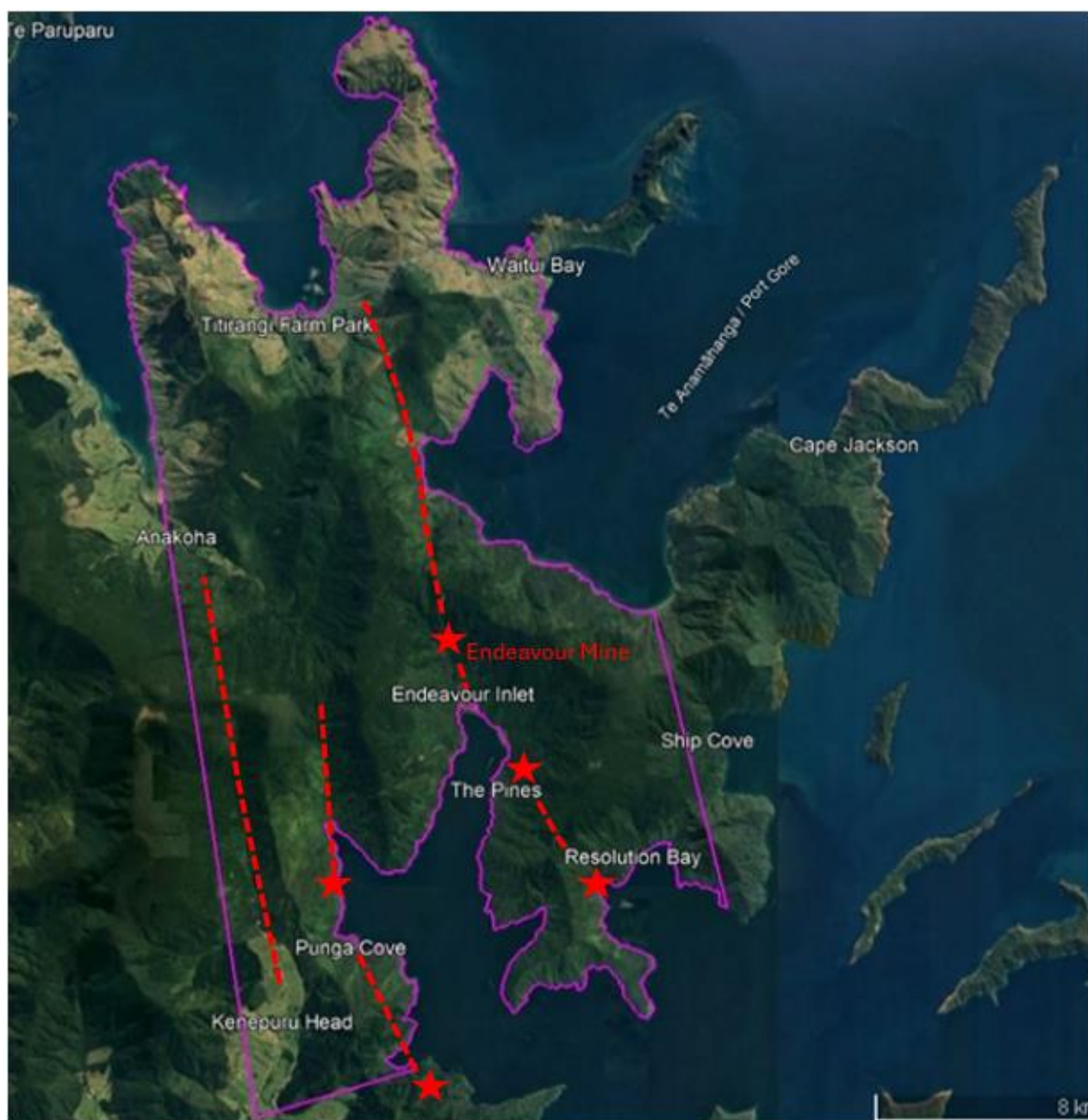
Figure 21. Exploration permit application (purple line), Potential shear zones (red dotted lines) and outcropping antimony mineralisation (red stars).
