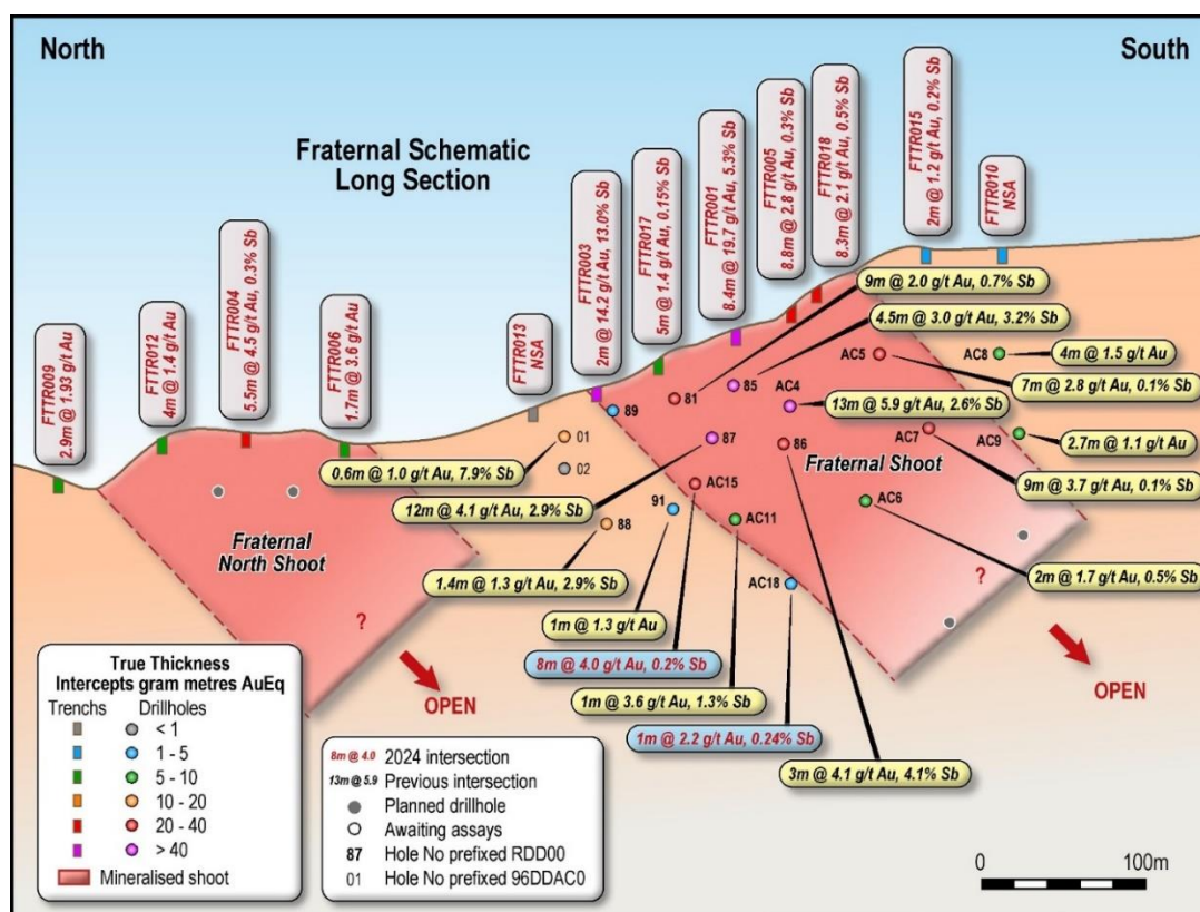
Figure 28. Fraternal schematic long section showing estimated true width intersections.
