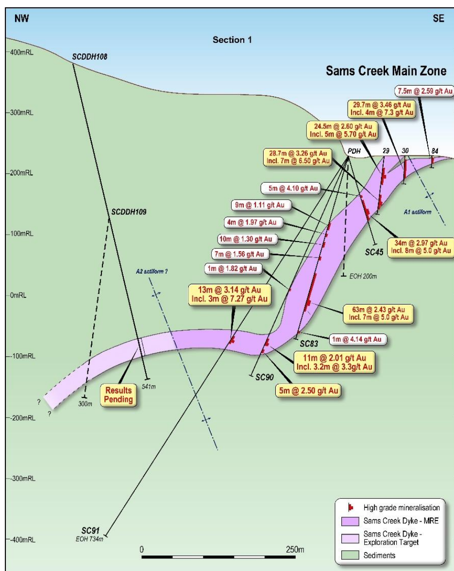
Figure 1: Schematic Cross-section 1 through the Main Zone mineralisation, showing SCDDH108 and planned SCDDH109 intersections.
