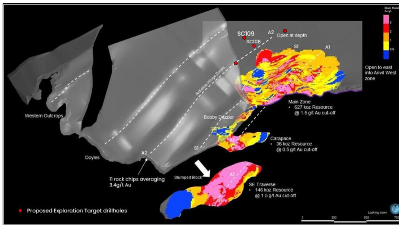
Figure 2: Plan view of undrilled SCD (grey) and MRE block model (magenta high grade, blue low grade).
