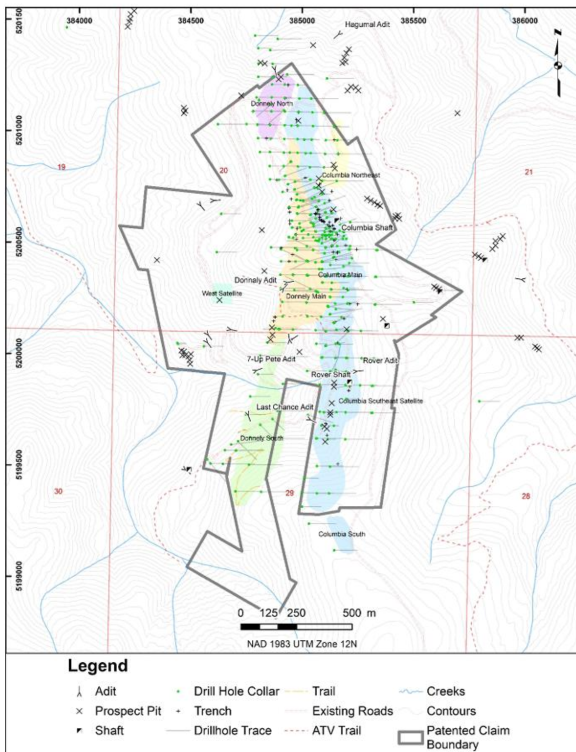
Figure 5 - Map showing the location of historical mining areas.
