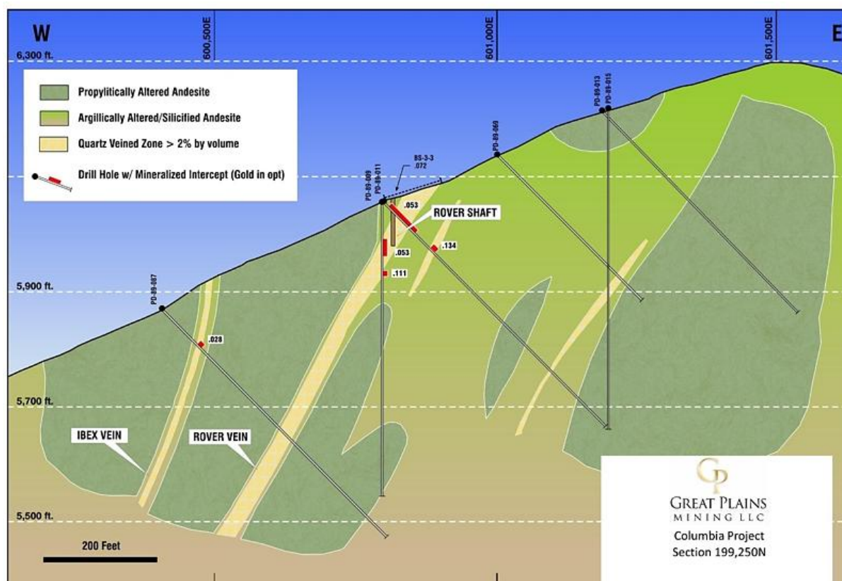
Figure 10 – Geology cross section showing the Rover Vein.
