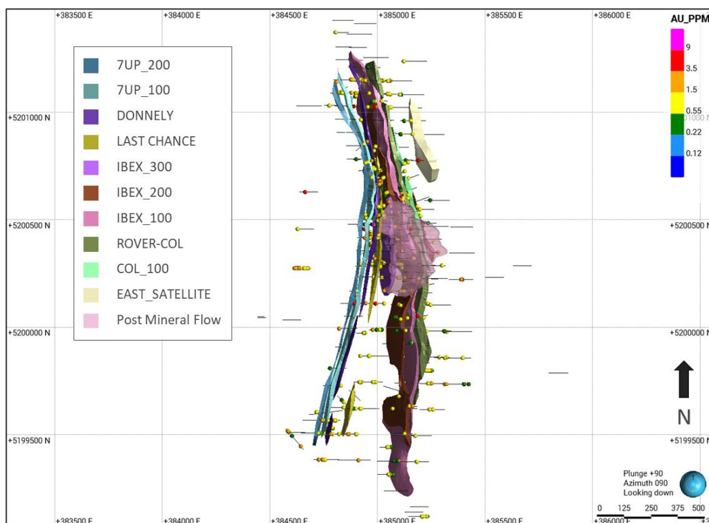
Figure 3: Plan view showing interpretative wireframes and additional mineralisation intercepts (K Kitchen, Independent Geologist Report 2025)
