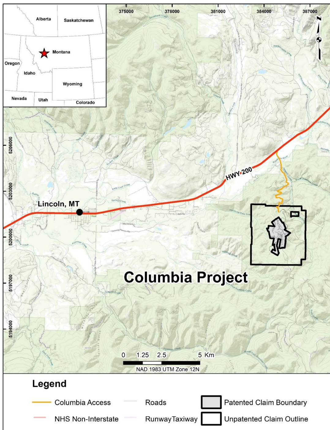
Figure 1 – Location and access to the Columbia Project.
