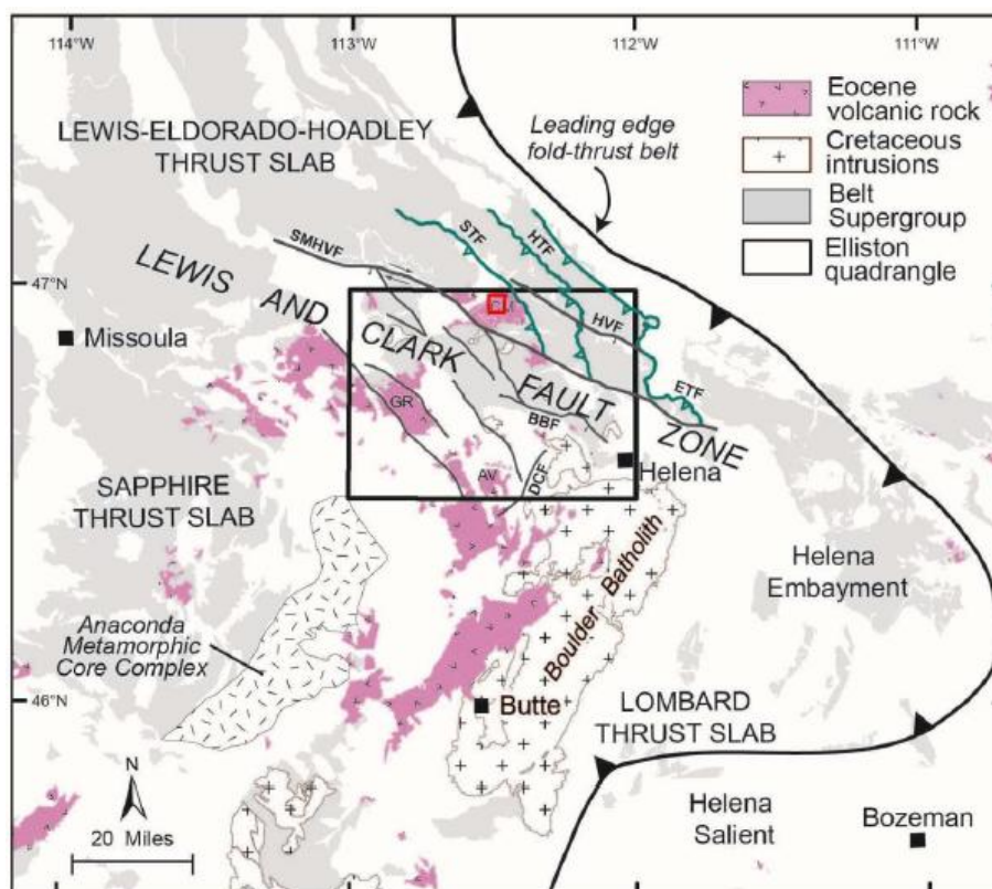
Figure 6 – Regional geology setting showing major faults of the Lewis and Clark Fault Zone (McDonald et al, 2020).
