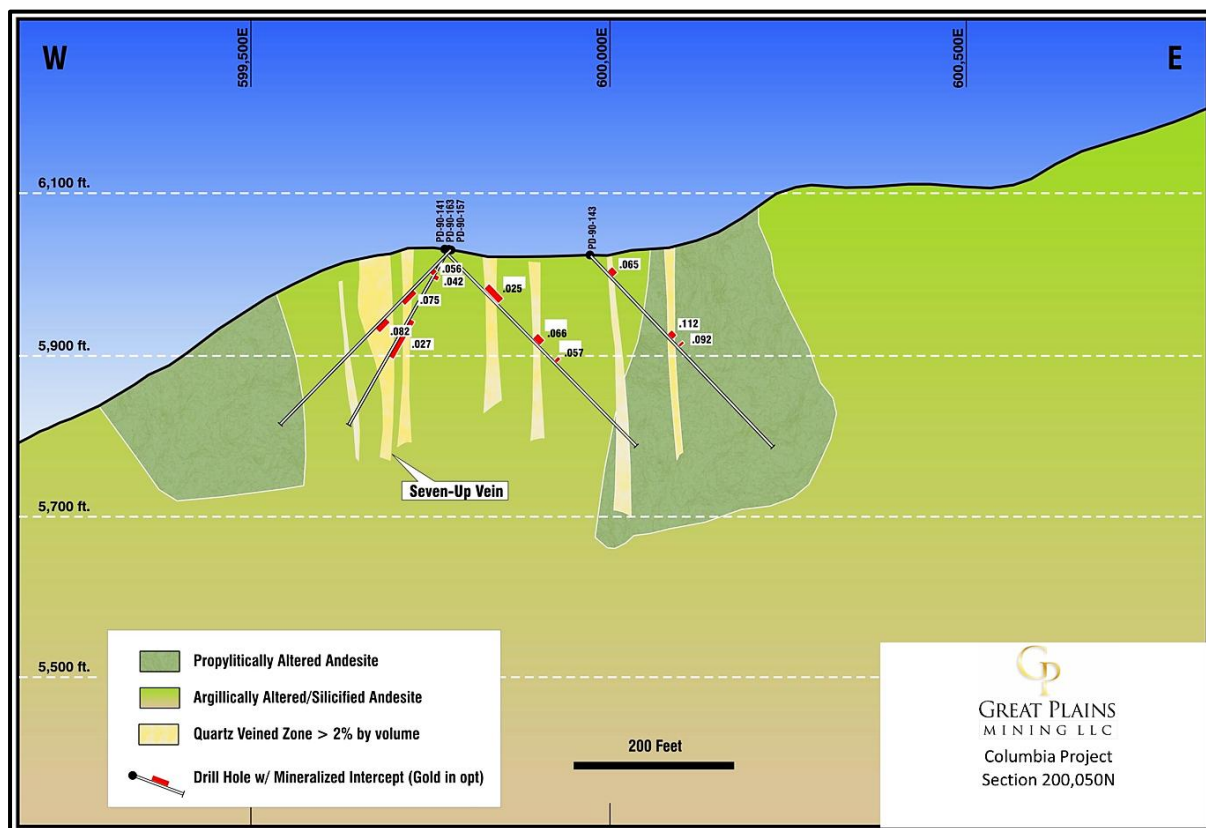
Figure 11 – Geology cross section for the Seven-Up Pete Vein.
