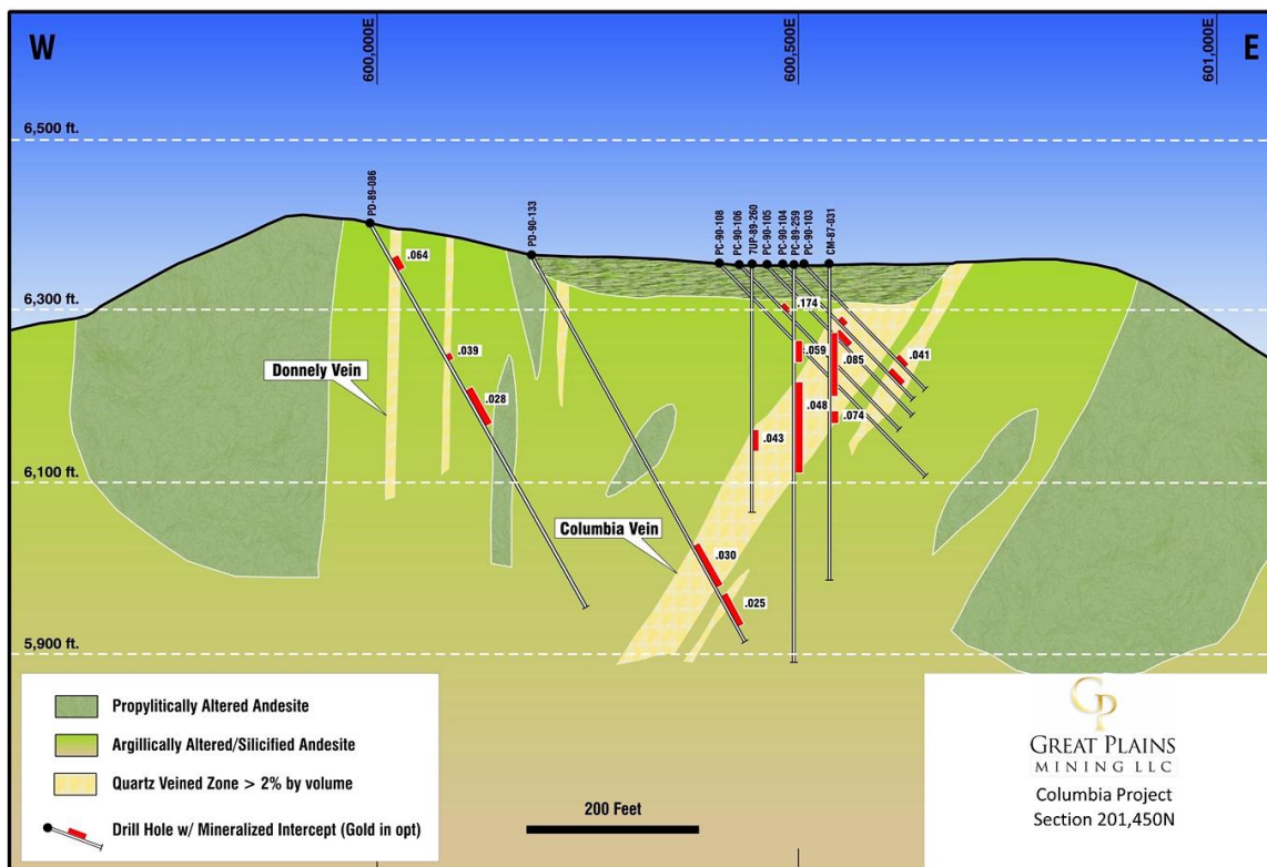
Figure 9 - Cross section showing the Columbia and Donnelly Vein geology.
