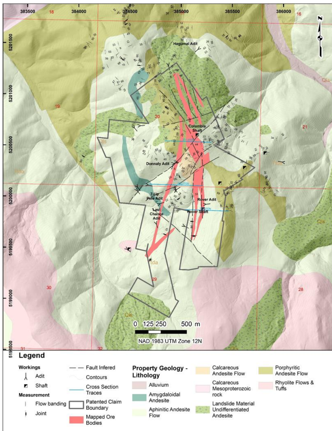
Figure 7 - Columbia Project property geology map.
