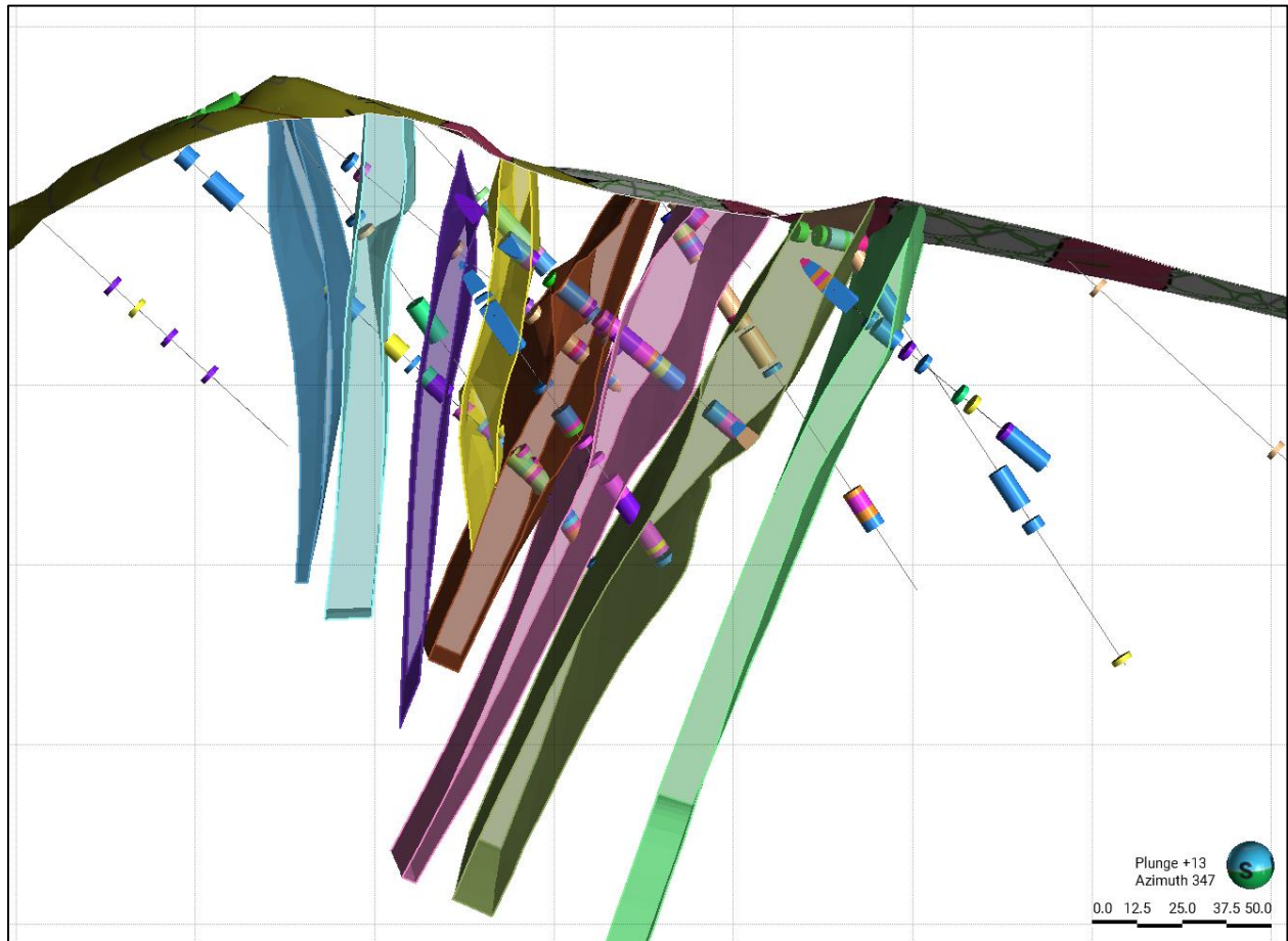
Figure 26 – Cross section looking north with a 40m window showing interpretative wireframes and vein logging. Vein logging colours.
