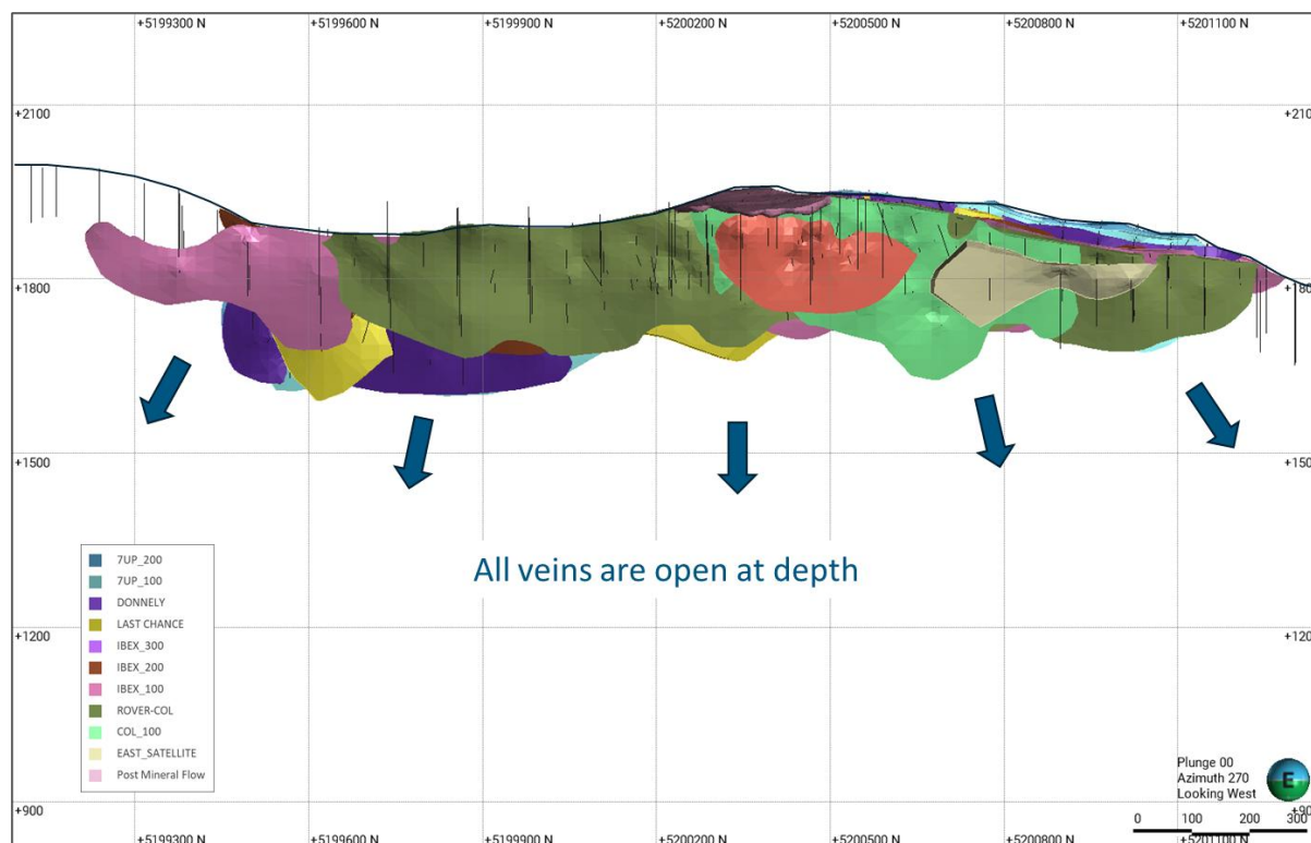
Figure 28 – Long section view looking west showing no drill testing below 300m with all veins remaining open.
