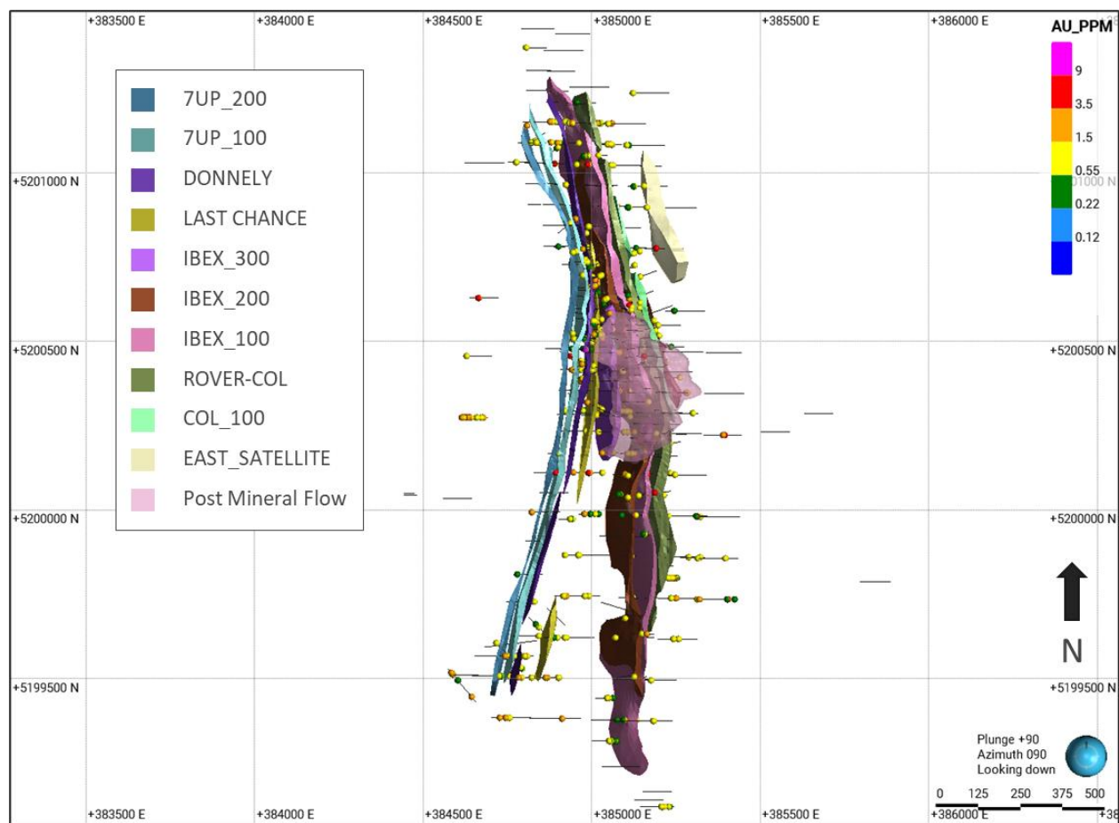
Figure 24 – Plan view showing interpretative wireframes and additional mineralisation intercepts.
