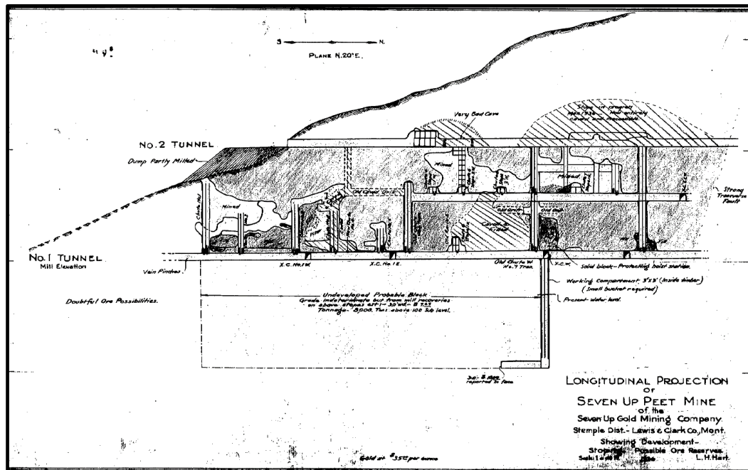
Figure 4 – Longitudinal projection dated 1936 showing historic development and stope.
