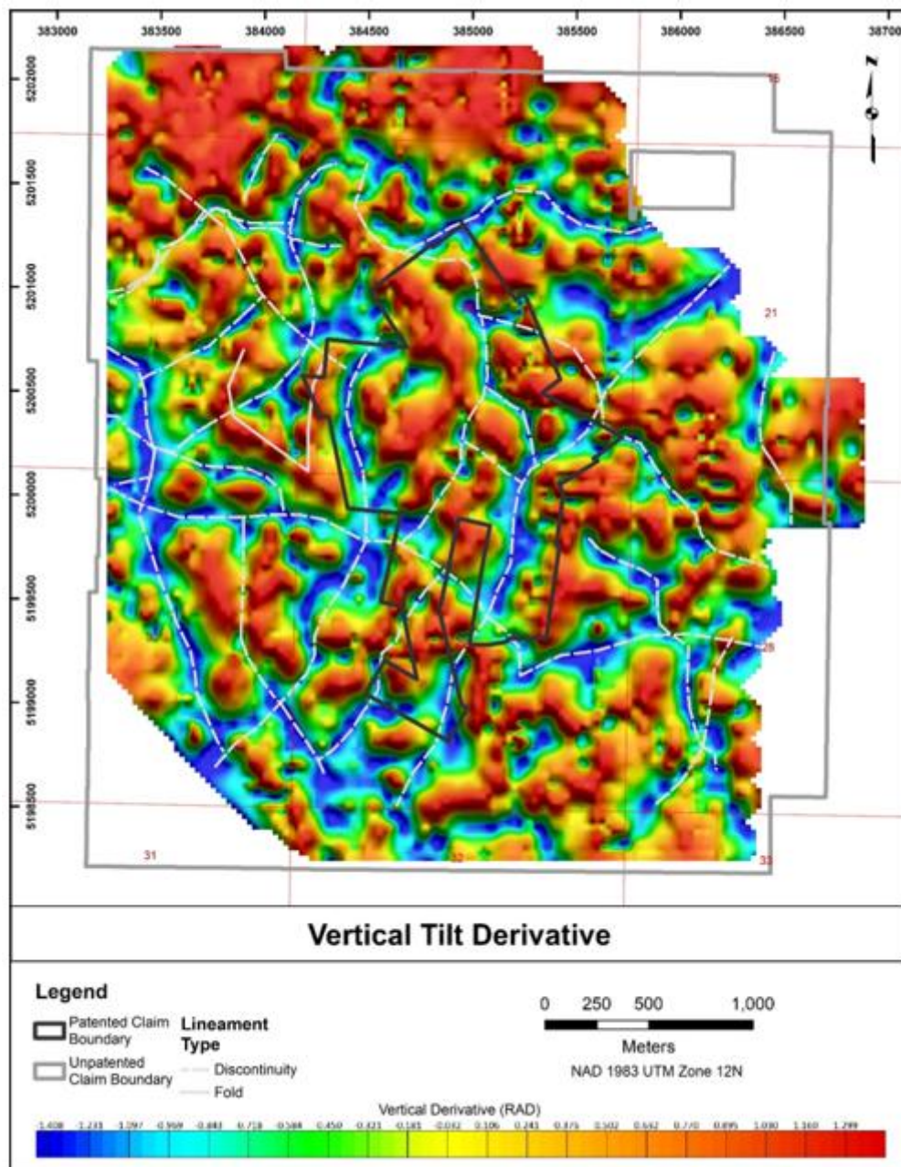
Figure 13 – Map showing the vertical tilt derivative overlaid with interpreted lineaments (Brewer, 2023).
