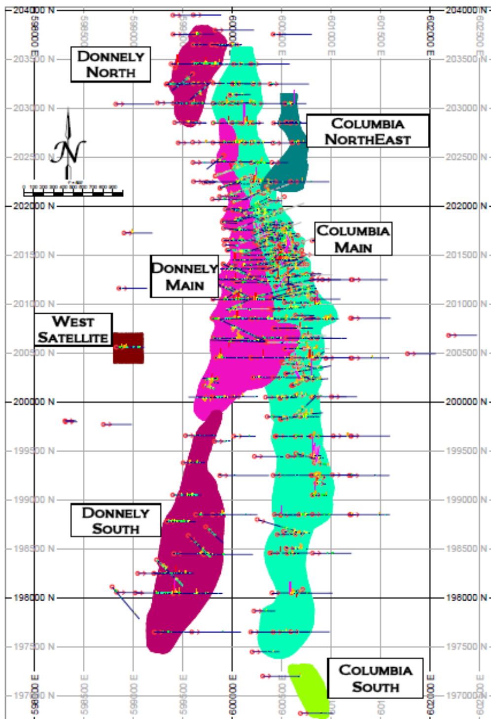
Figure 8 – Map showing the location of the Columbia Project individual deposits.
