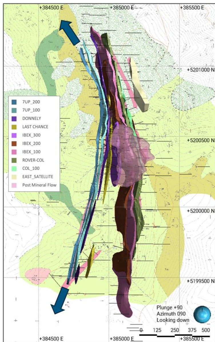
Figure 27 – Plan view showing interpretative wireframes over mapped geology with drill traces black lines. Blue arrows indicate where 7UP_100 and 7UP_200 veins are untested along strike.
