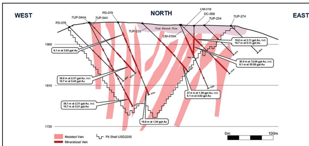
Figure 22 – Example cross-section at 5,200,480mN showing the modelled veins in red, significant assays from drillholes and the RPEEE pit shell in black.
