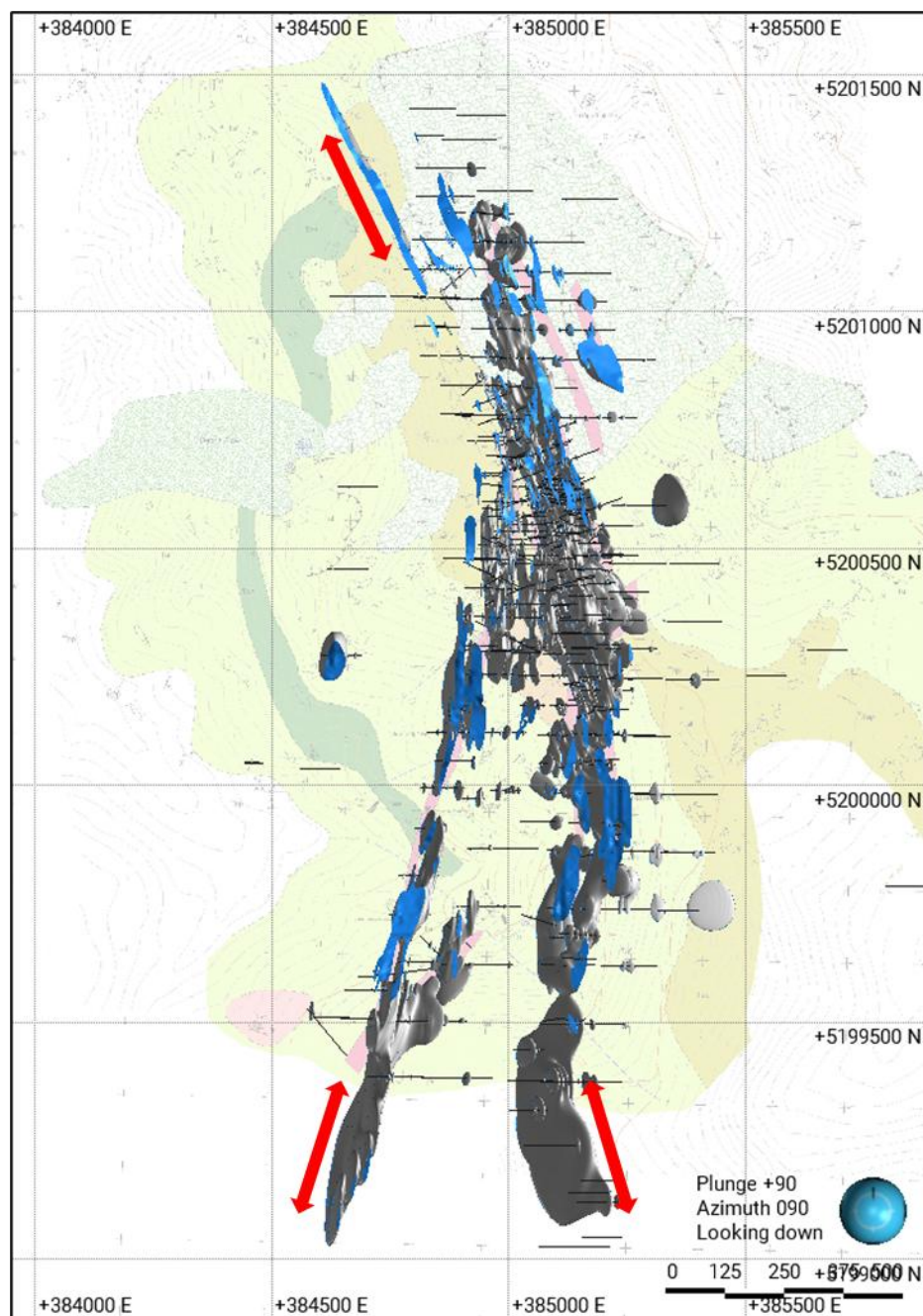
Figure 30 – Plan view of the Mining Plus generated mineralisation shapes at 0.3ppm Au for determination of an exploration target. Red arrows indicate extension zones for the 7UP and IBEX veins.
