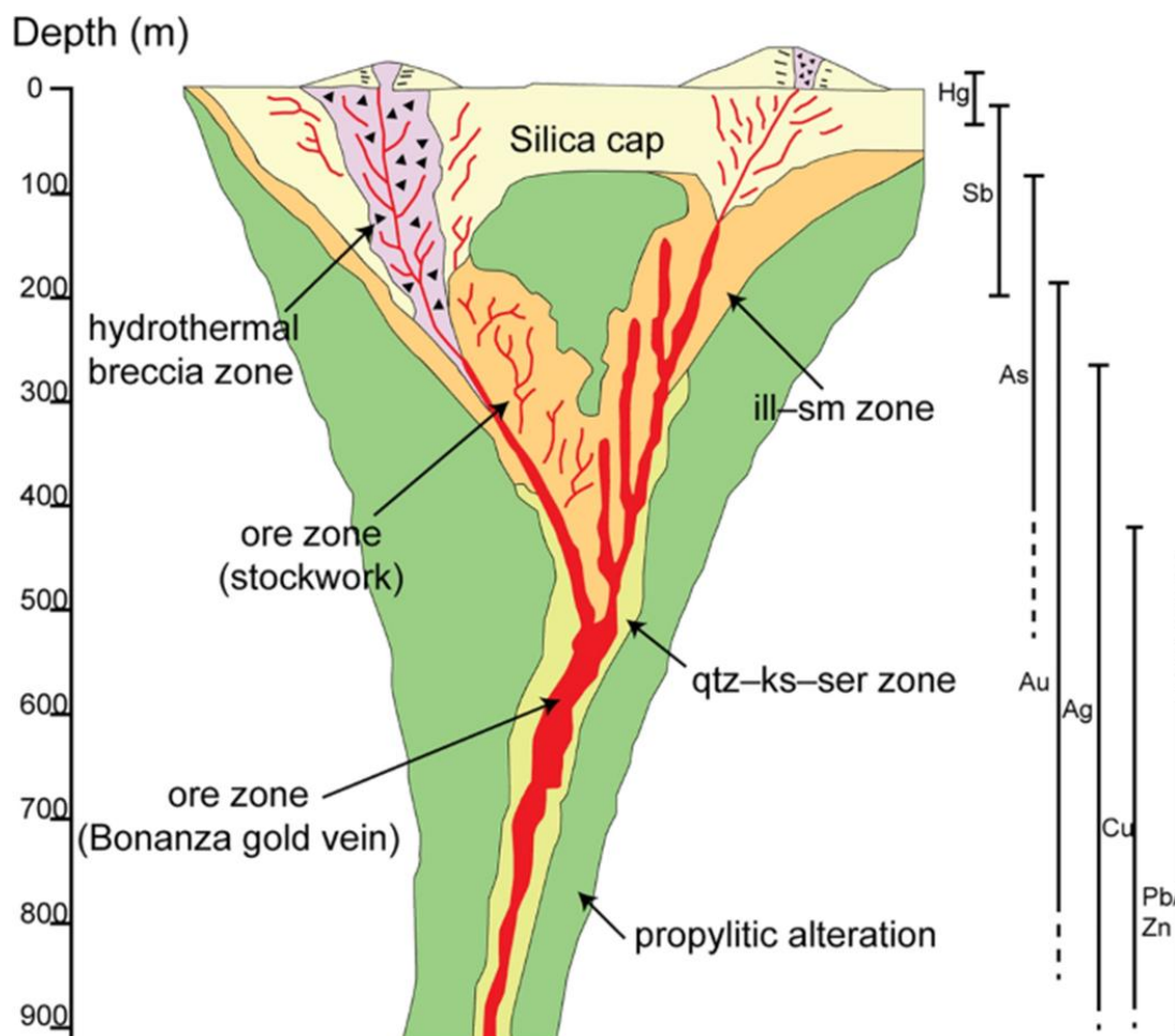
Figure 29 – Schematic section from Kaewpaluk et al, 2024 highlighting the alteration and geochemical zonation in a low-sulphidation epithermal system.
