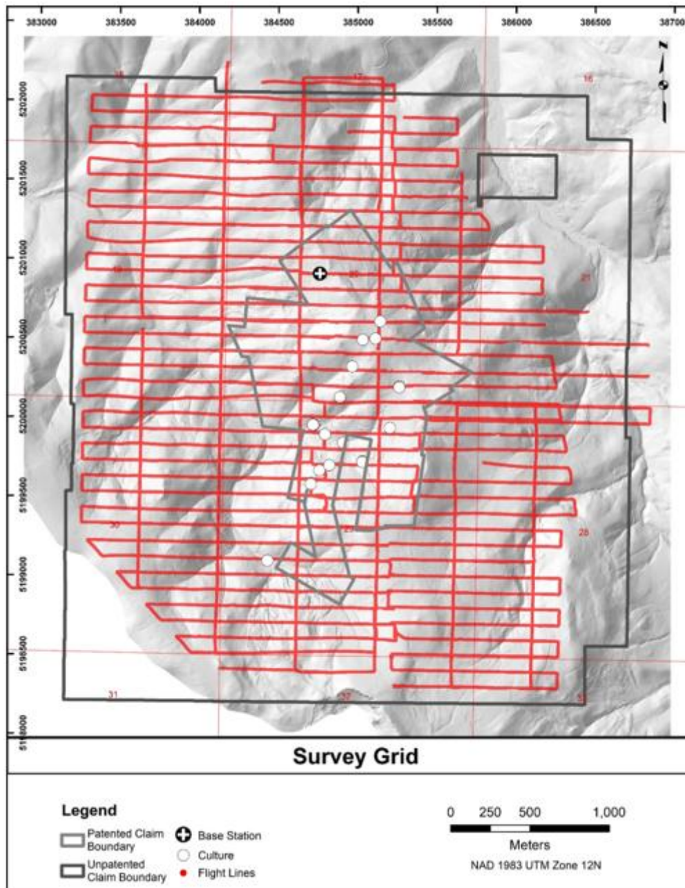
Figure 12 – Layout showing drone magnetic survey lines (Brewer, 2023).
