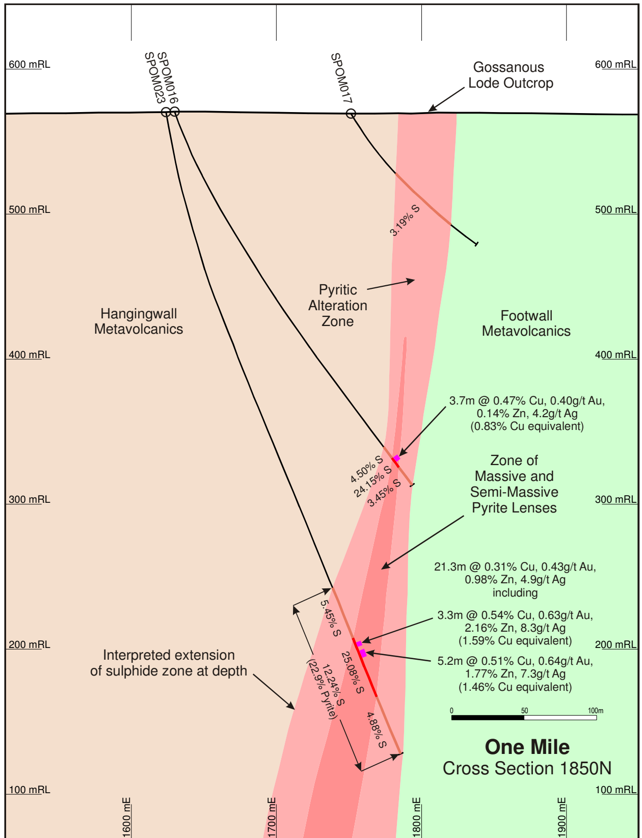
Figure 2. Interpreted geological cross-section 1850N on the One Mile Mining Lease showing the most recent drilling at the southern end of the area. The drilling shows an increase in grade and width of the sulphide zone at depth and to the south. The bottom 124m of hole SPOM023 which averages 12.24% sulphur (equivalent to 22.9% pyrite) indicates the increase in width of the enclosing alteration zone associated with the mineralisation.
