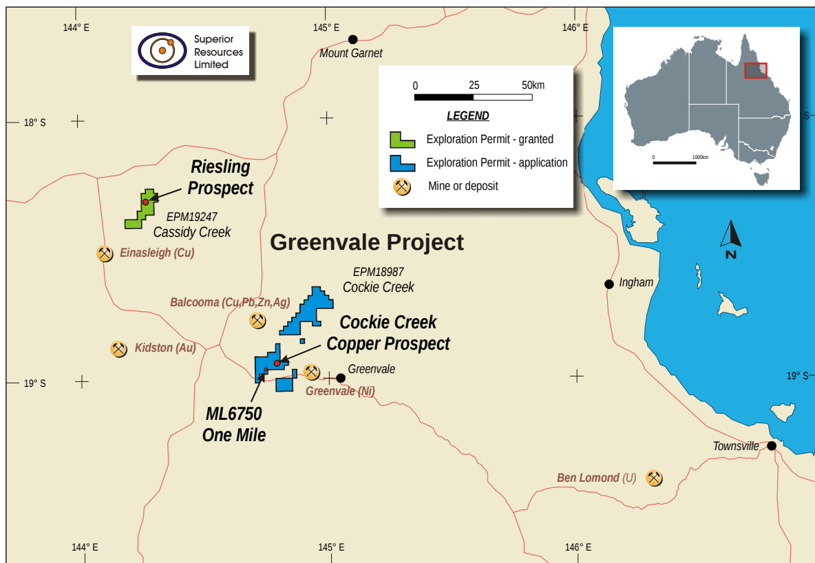
Figure 1. Location of Superior's Greenvale Project and One Mile Mining Lease in northeast Queensland
