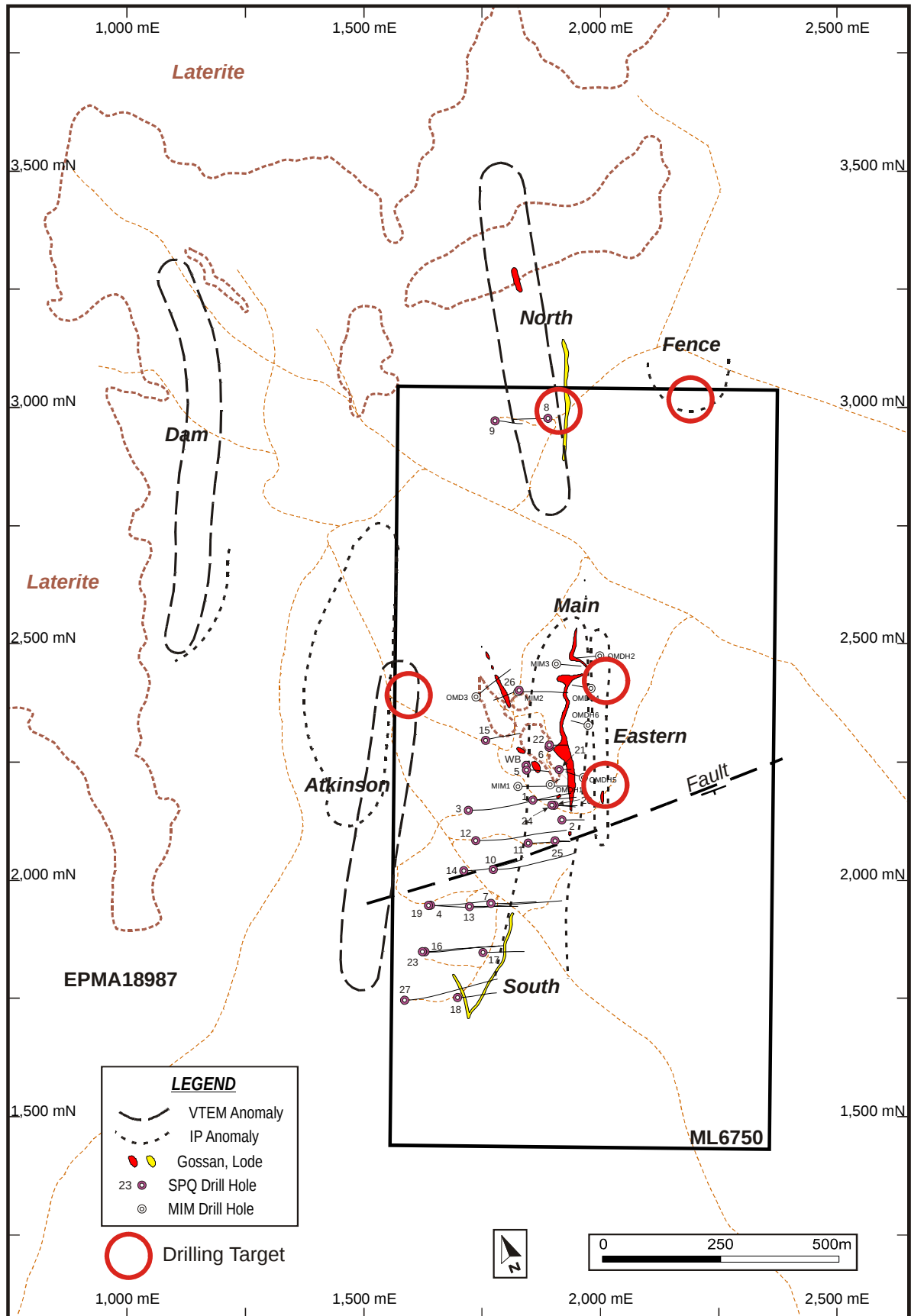
Figure 2. One Mile Mining Lease showing the geophysical targets and the areas proposed for drilling in the current program.
