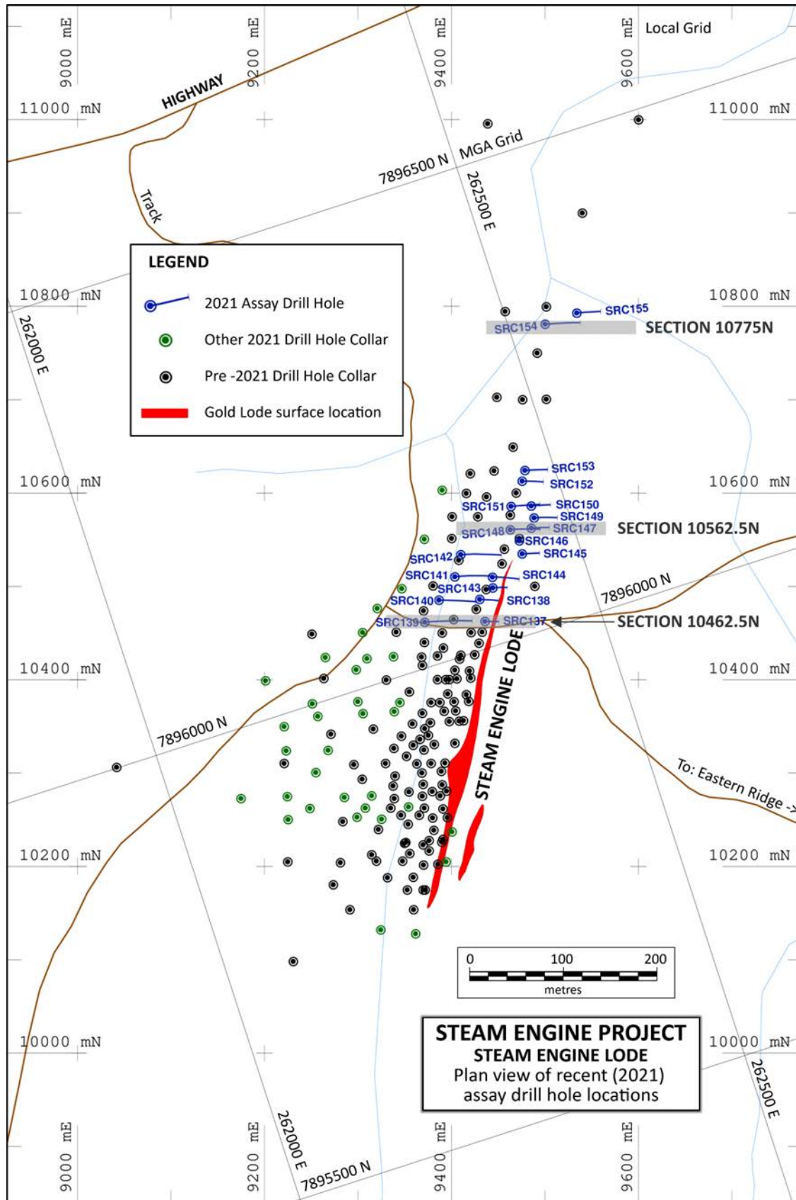
Figure 7. Plan showing drill hole collar locations at the Steam Engine Lode and hole traces of RC holes reported in this announcement.
