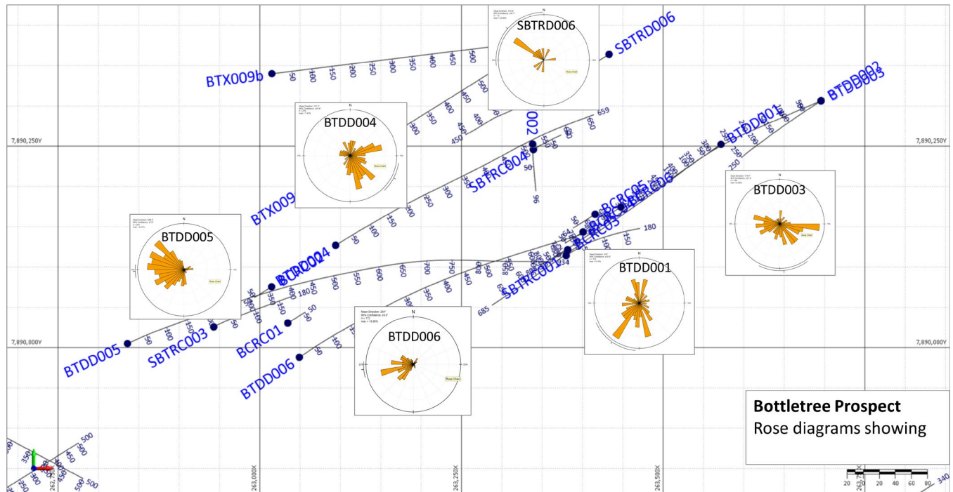
Figure 6. Current drill hole plan showing rose diagrams of mineralised vein structures within diamond core holes. The rose diagrams indicate dip direction frequency distributions.
