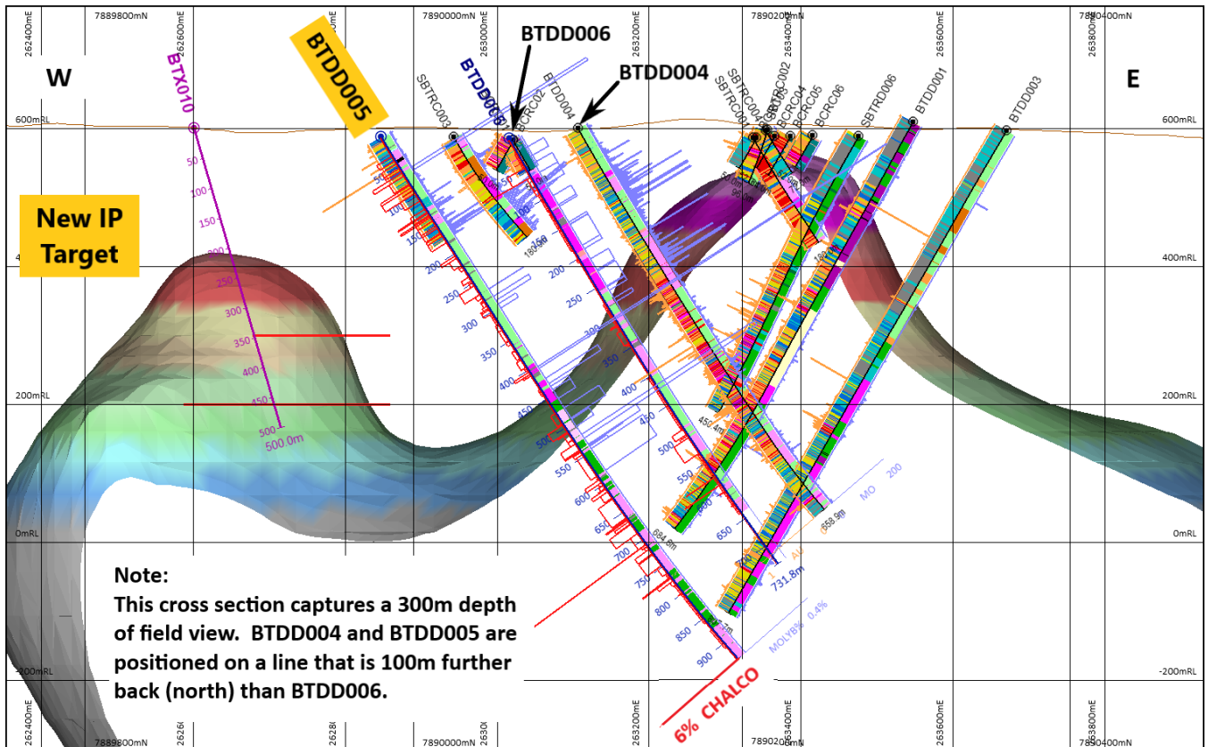
Figure 1. E-W cross section capturing a 300m depth of field view showing 20mV/V IP chargeability iso-surface of new 3D IP model, part of newly identified IP chargeability anomaly and holes drilled to date. Visual estimations of chalcopryite and molybdenite are presented as histograms (where assays are not available) on each side of drill hole traces.
