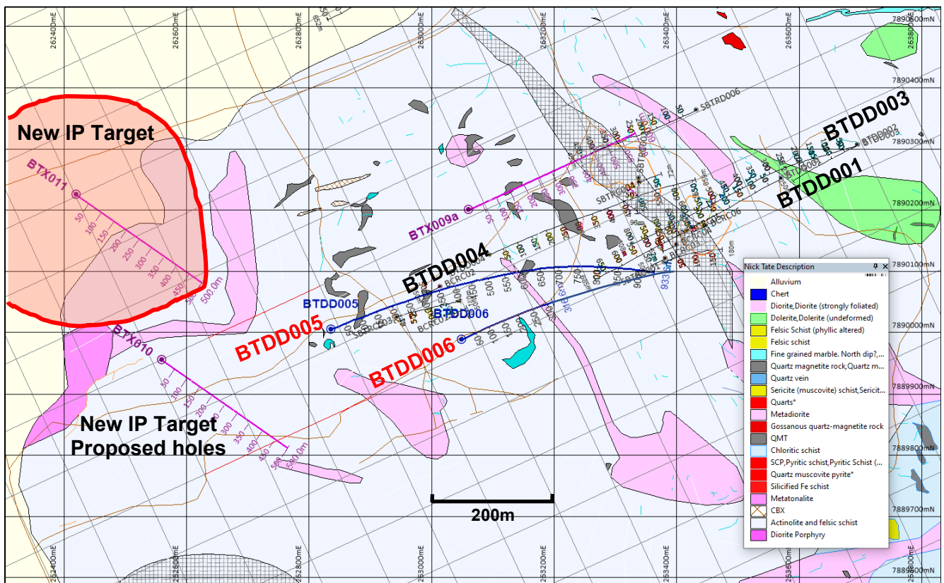
Figure 2. Surface geology plan showing collar locations, drill hole traces for BTDD005, BTDD006 and 2021 drill holes (in black) and approximate position of the newly identified IP chargeability target.
