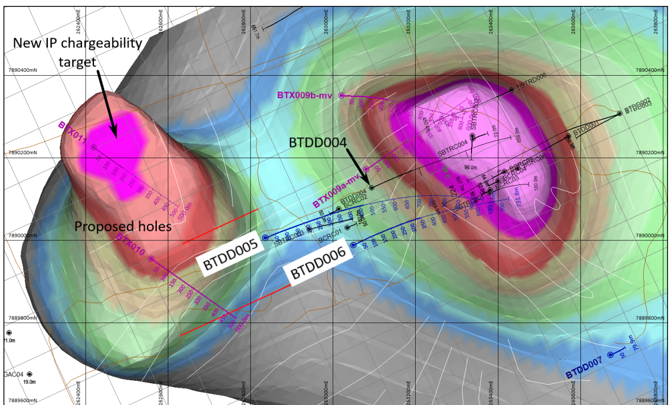
Figure 4. Revised 3D IP chargeability model showing the newly identified IP chargeability anomaly in the west and the original IP chargeability anomaly to the east. Viewed looking downwards and towards the north.
