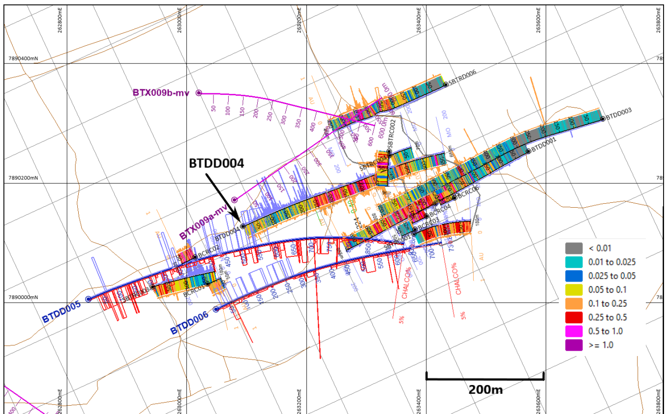
Figure 5. Plan of current drill holes. Individual metre copper and gold grades are shown for assayed holes. Where final assays are yet to be received, visual estimates of chalcopyrite and molybdenite are shown in histogram format.
