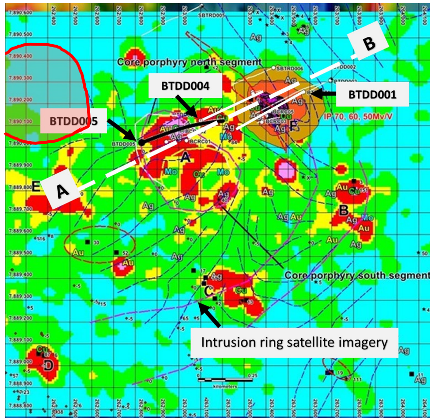
Figure 3. Gridded soil copper geochemistry showing select drill holes, satellite imagery interpreted intrusion ring; profile section A-B and approximate position of the newly identified IP chargeability target. Porphyry targets are shown, labelled A to F.
