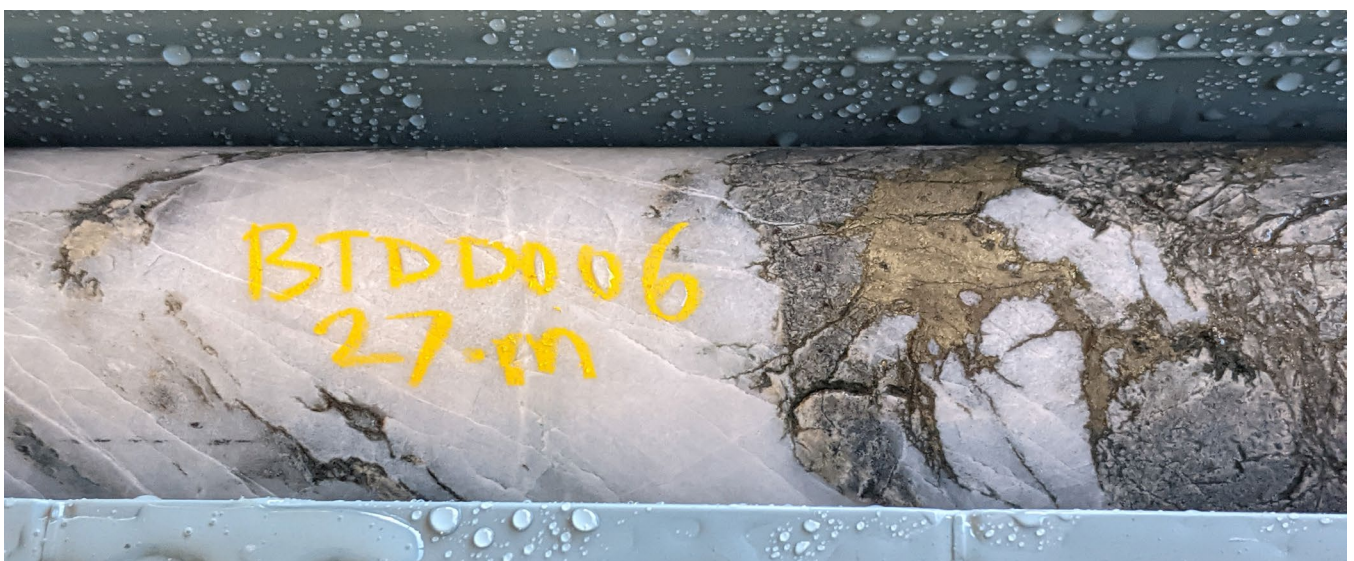
Figure 9. BTDD006 – 27m – chalcopyrite infill in buck quartz vein.
