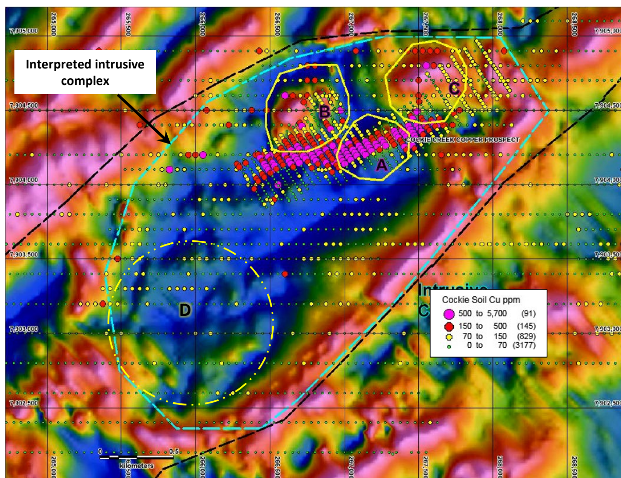
Figure 10. Cockie Creek thematic Cu soil data and interpreted porphyries on TDr VI NSSF processed airborne magnetics data, showing interpreted porphyry intrusions (A to D) within an interpreted intrusive complex.
