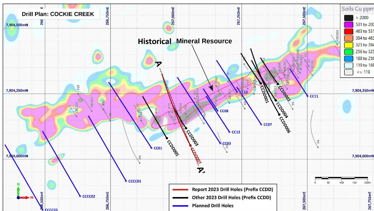
Figure 9. Plan map of the Cockie Creek Discovery Outcrop area showing completed drill holes CCDD001 – CCDD007 (in black) with new assay data discussed in this release (in red), other 2023 drill holes reported in previous releases (in black), planned but not yet drilled holes (in blue) and historic drill holes (in grey) over gridded Cu soil geochemistry. Outline of historic Mineral Resource at surface and cross section A-A' is shown.
