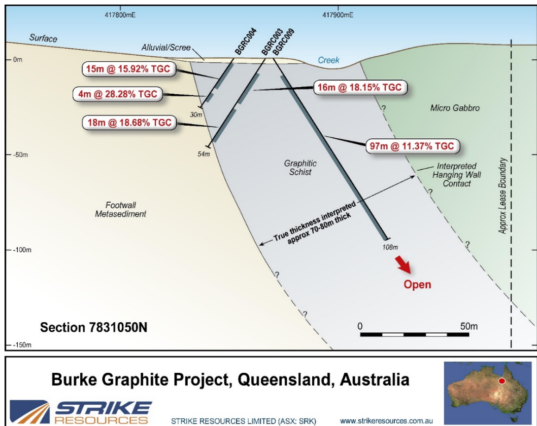
Figure 3 - Drillhole Cross Section 7831050mN
