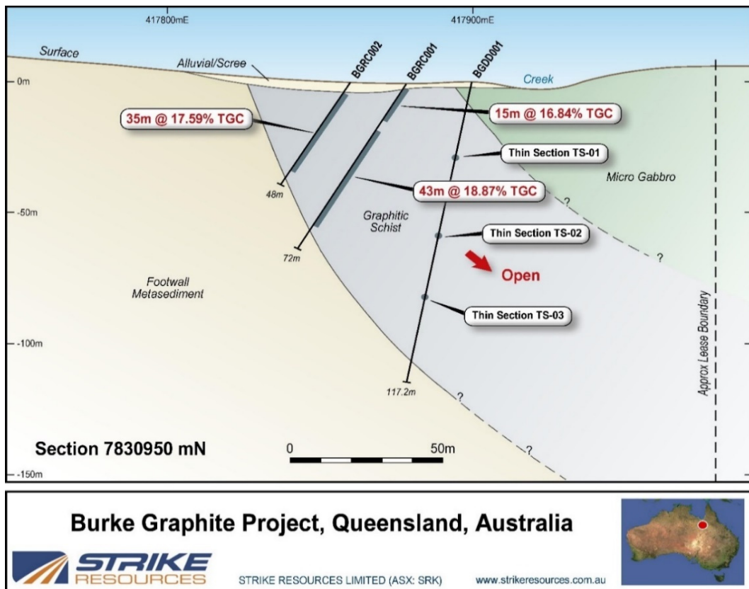
Figure 2 - Drillhole Cross Section 7830950mN
