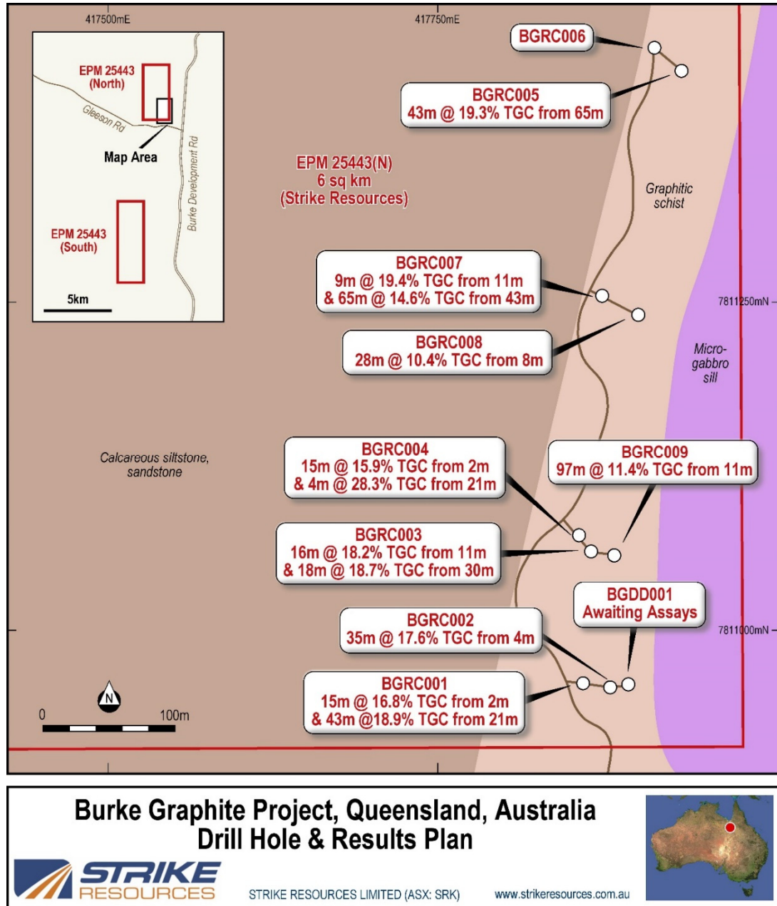
Figure 1 - Location Plan for April/May 2017 Drilling
