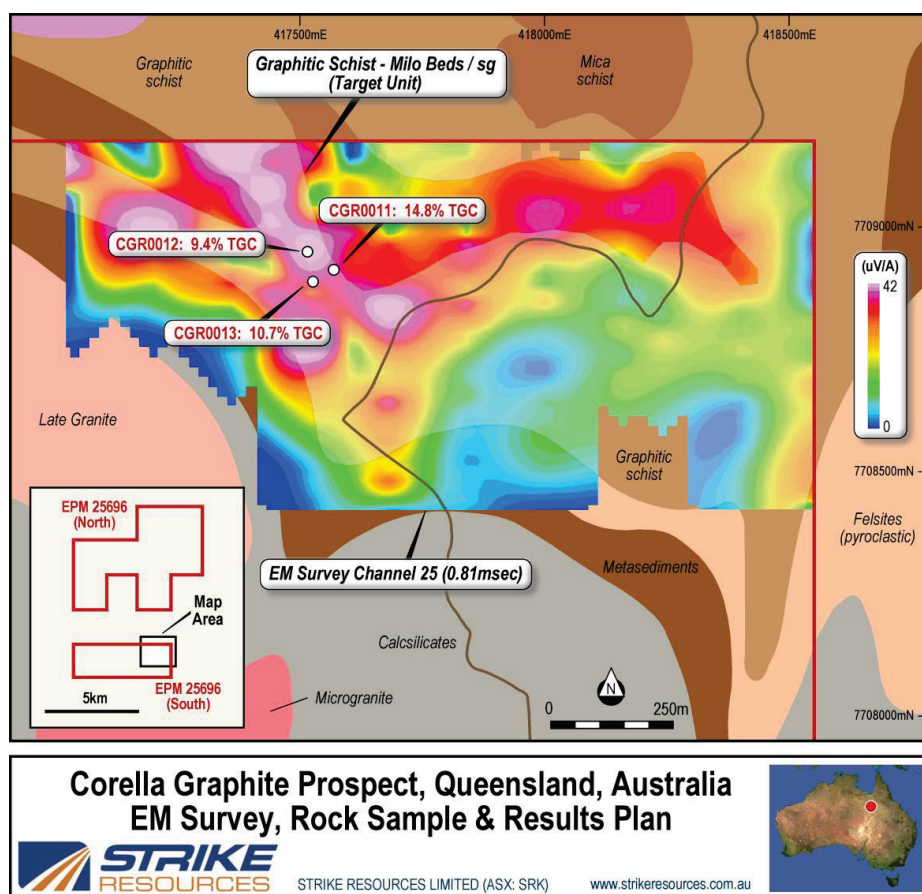
Figure 4 - EM Survey - Corella Prospect, Burke Graphite Project
