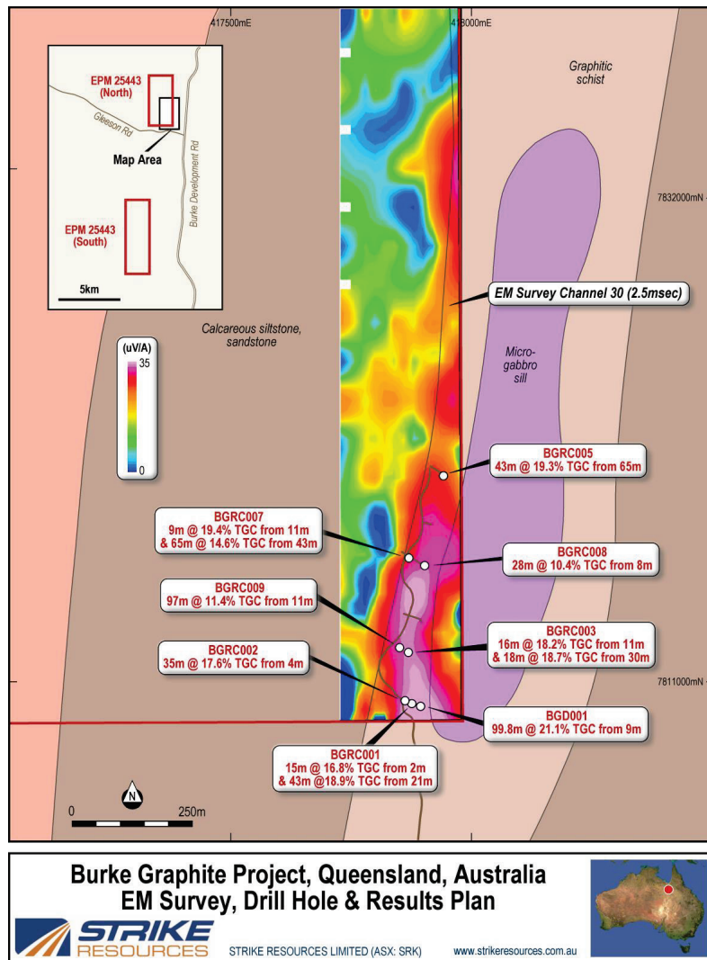
Figure 5 - EM Survey - Burke Prospect, Burke Graphite Project
