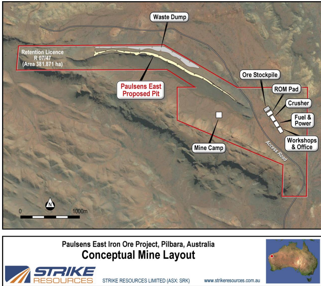
Figure 4: Conceptual Mine Layout of Paulsens East Project
