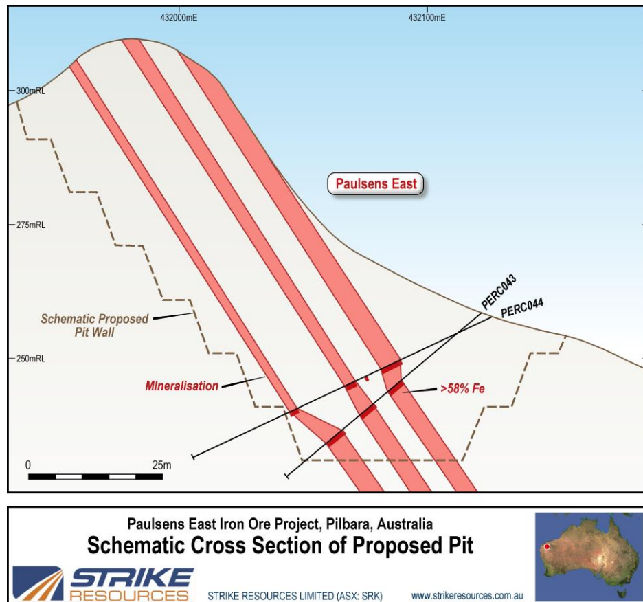
Figure 5: Schematic Cross Section of proposed pit at Paulsens East
