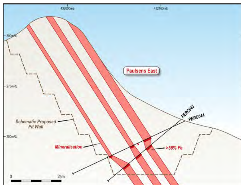
Figure 11: Conceptual Mine Layout of Paulsens East Project
