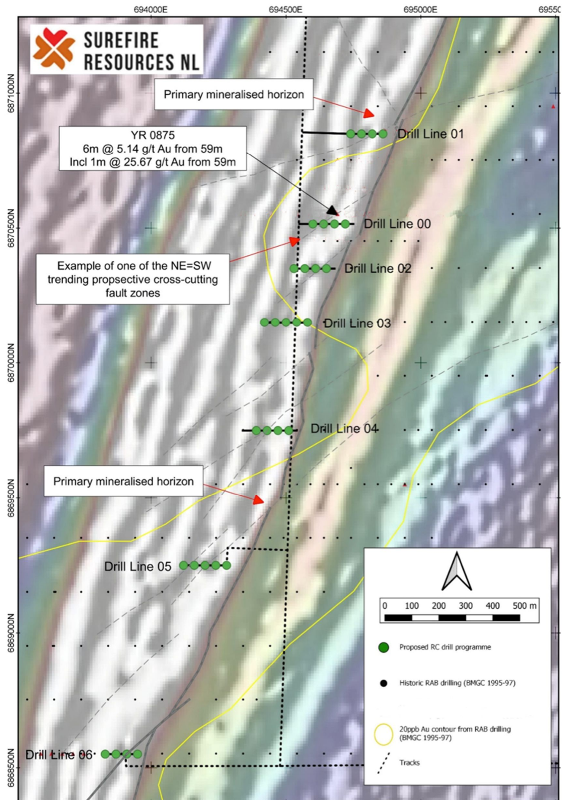
Figure 2: Proposed RC drill programme to target the main NNE trending gold bearing horizon and NE-SW cross-cutting fault zones.
