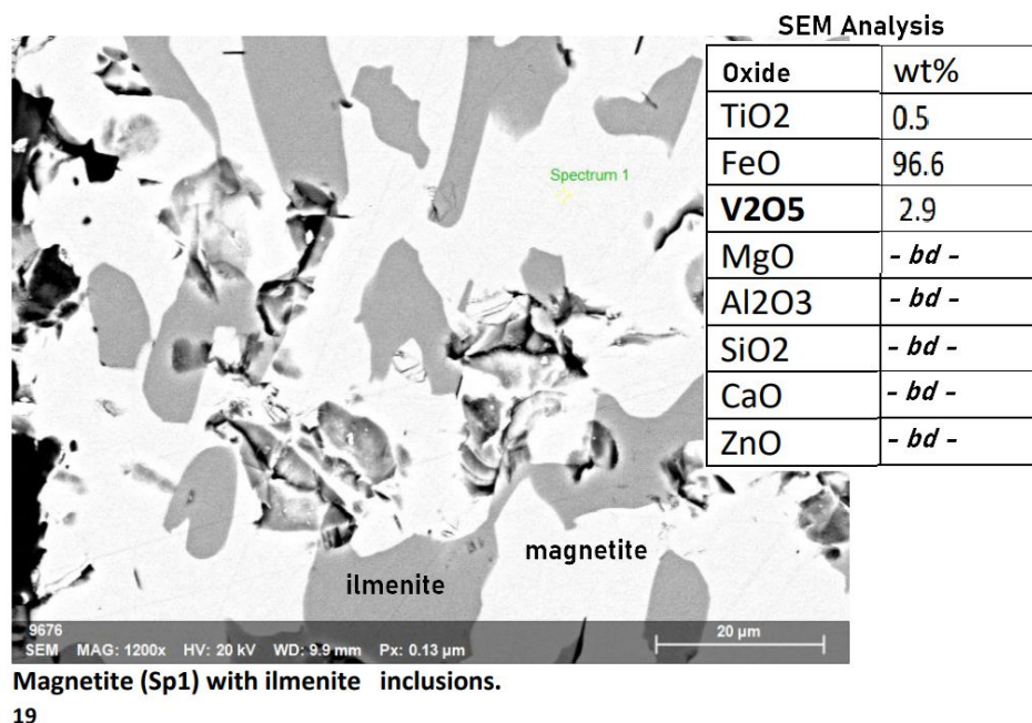
Figure 2 Image of ilmenite exsolution lamellae in magnetite with magnetite mineral analysis sample VBRC018 – Main Lode - Hole coordinates, x=695024 y=6782048 from 126m to 127m, 1m @ 0.8% \text{V}_2\text{O}_5 (- bd - = below detection)
