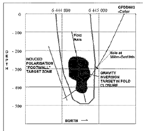
Section showing design and current position of the Goldfinger DDH03
