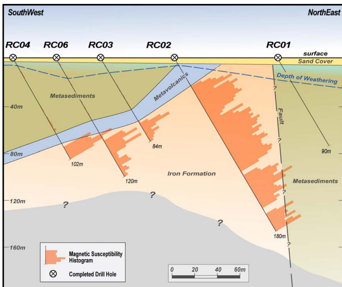
Figure 2 Interpretative Geological Drill Section – Hicks Hill
