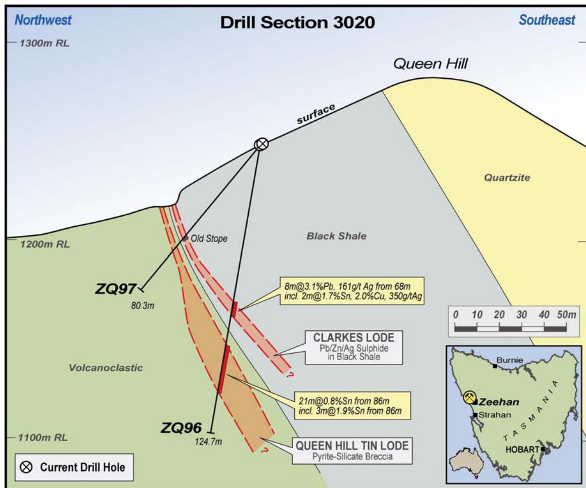
Figure 2. Queen Hill Interpretative Geology Across Section 3020
