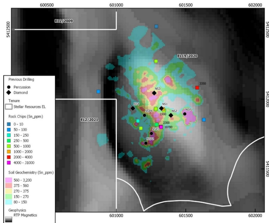
Figure 2 - North Scamander Tin-Base Metals Advanced Prospect - Regional Magnetics RTP (greyscale), Surface Soil Geochemistry, and Historic Drillholes, EL19/2020 (GDA94 Grid)
