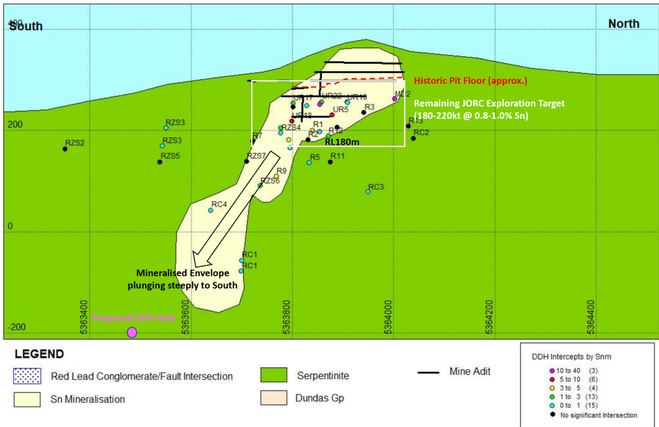
Figure 10 – Razorback Mine Tin Deposit Long Projection showing Planned Hole
