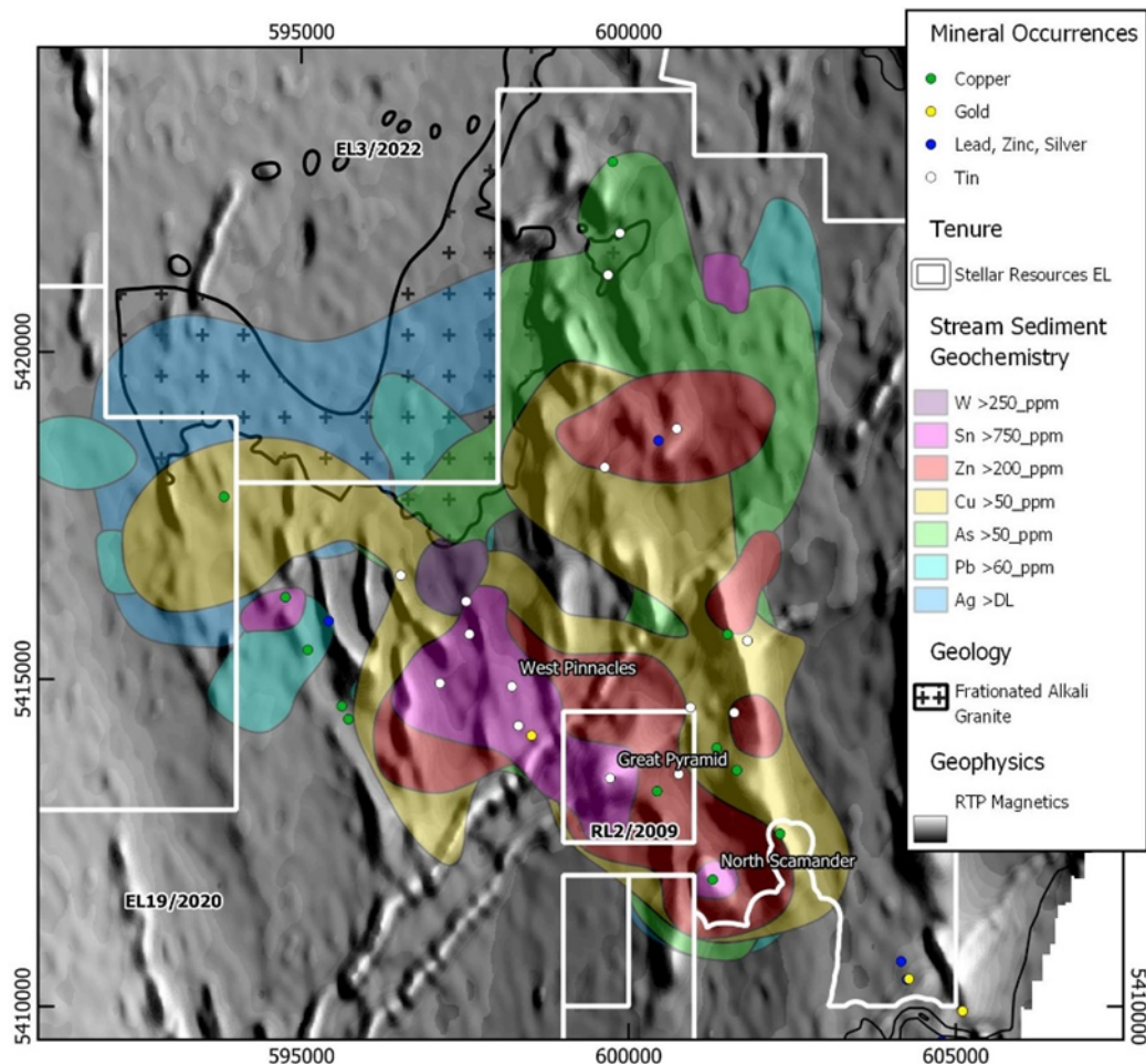
Figure 1 – Scamander District - Regional Magnetics (greyscale), Surface Stream Sediment Geochemistry, Mineral Occurrences, and Outcropping Fractionated Alkali Granite over EL19/2020 (GDA94 Grid)
