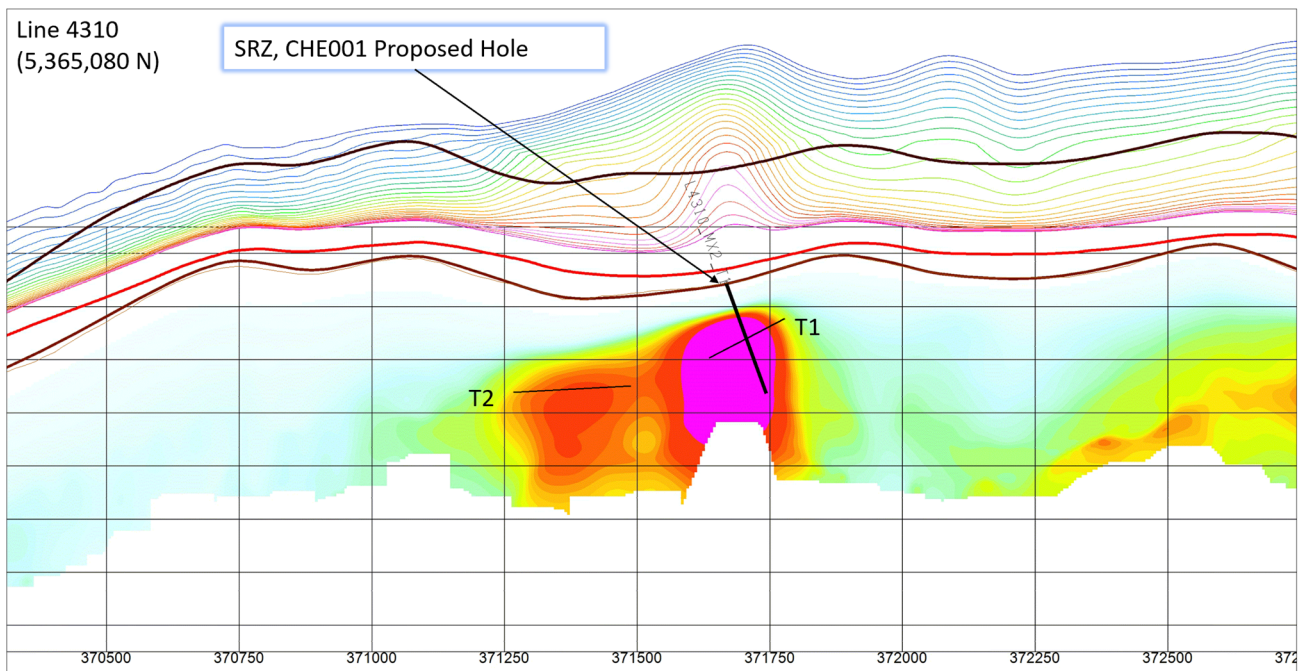
Figure 7 – Carbine Hill East Prospect Cross Section, Flight Line 4310 (5,365,080 N) Resistivity Depth Image (RDI), Surface Topography (brown line), EM TAU dB/dt Z Profile (above topography), Modelled Plates and Proposed Drillhole (Source: EL22/2010 Yunnan Tin 2015 Annual Report, Appendix 5)
