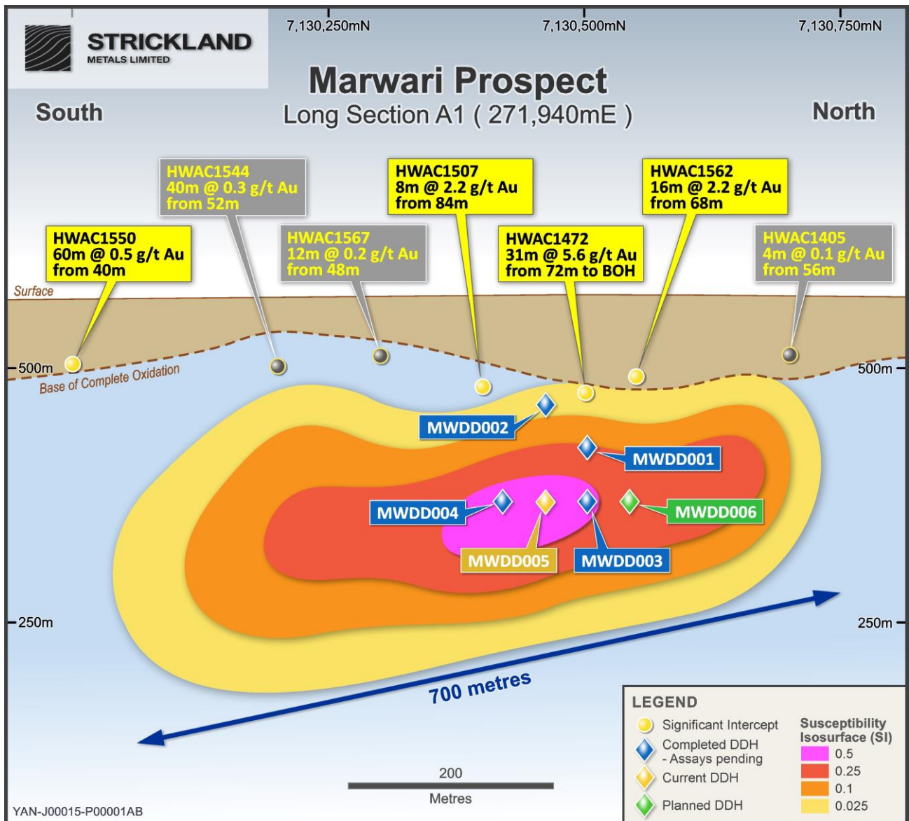
Figure 1: Marwari Long Section (looking west): Highlighting the completed, current and planned diamond drill hole intercept positions, in relation to the modelled magnetic inversion model and previously reported aircore assays.
