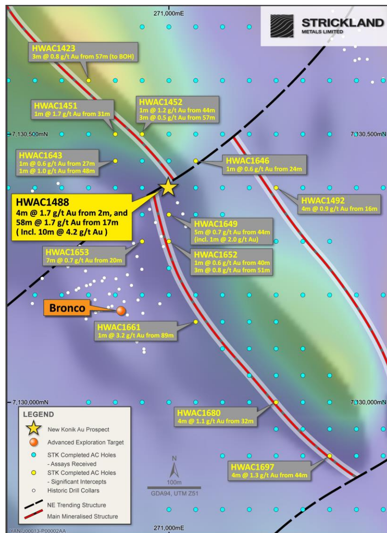
Figure 7: Topographic image showing Konik aircore anomalism
