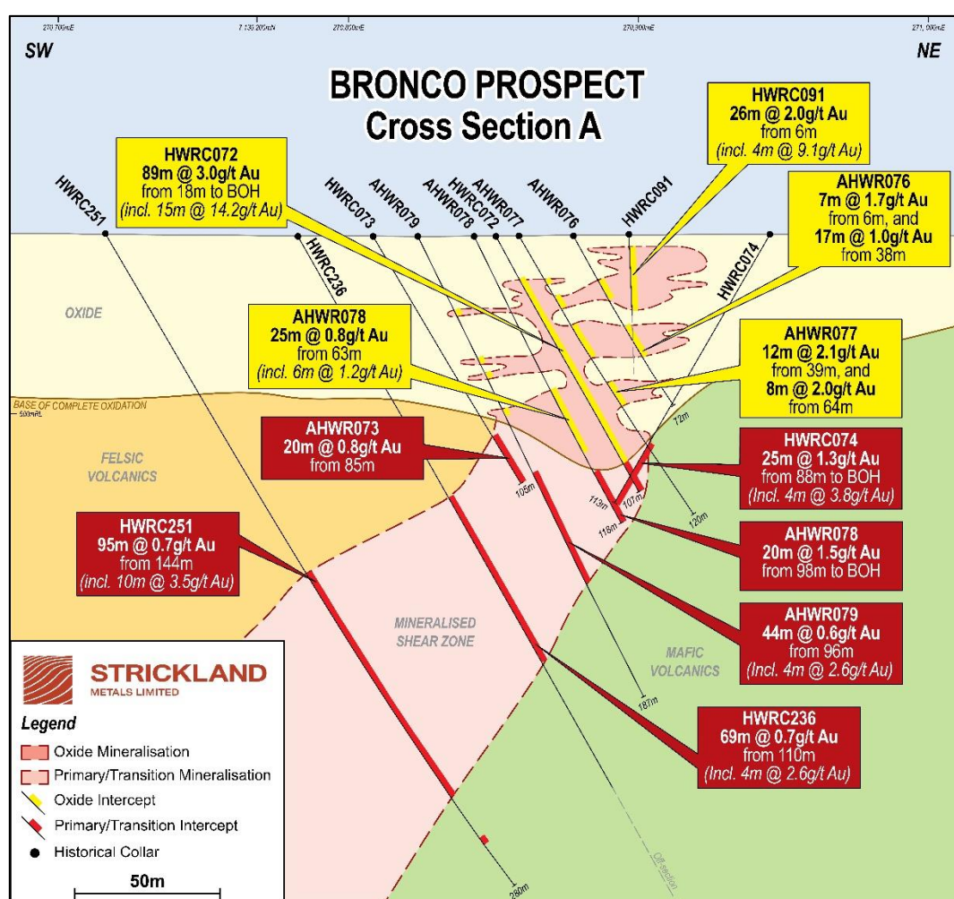
Figure 2: Cross section of Bronco-Konik highlighting shallow high grade oxide intercepts and primary bulk potential
