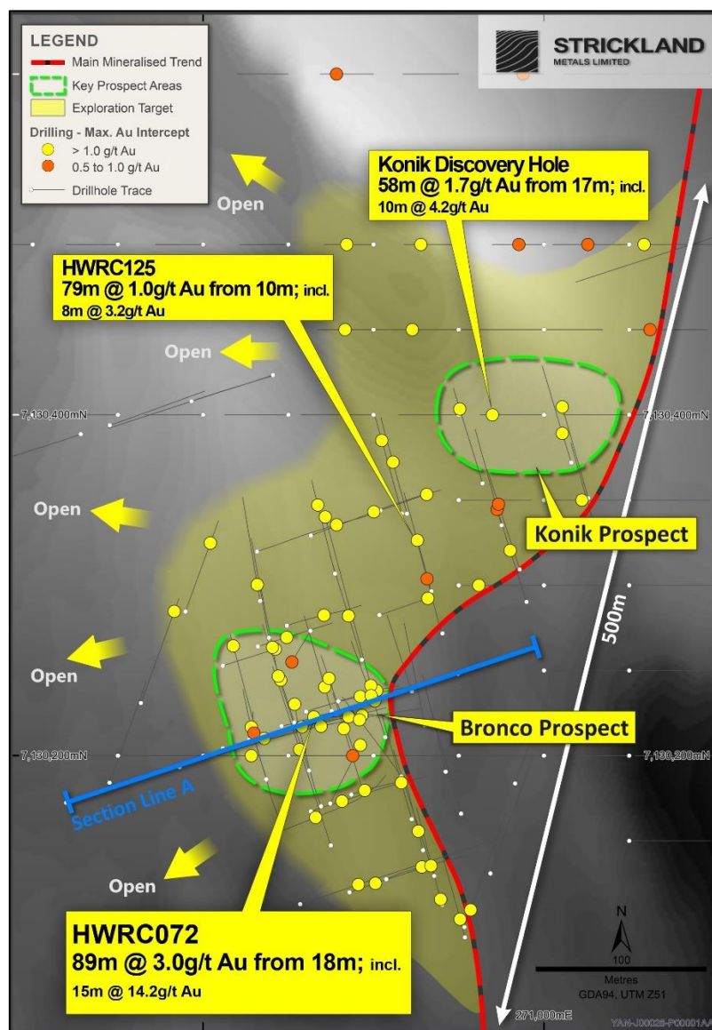
Figure 1: Topographic image showing the connection between the Bronco and Konik prospects
