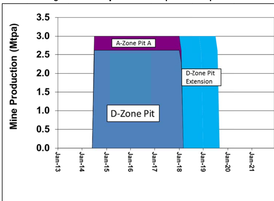
Figure 6: Development Case A production profile
