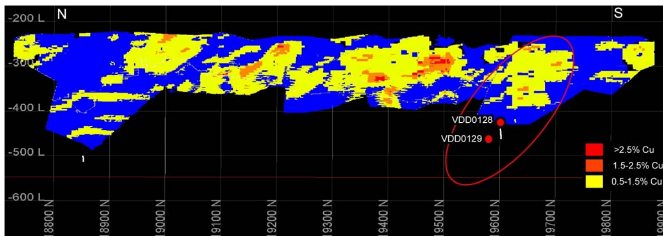
Figure 17 – Long sectional view of the D Zone Mineral resource displaying the distribution of copper grade (Mineral Resource not updated with the results from VDD0128 and VDD129. Surface RL = -230m to -250m).
