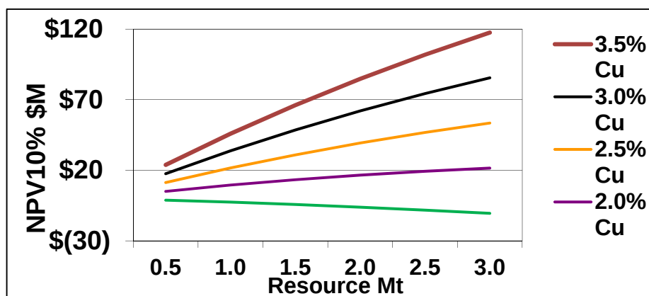
Figure 8: Impact of the additional material at various grades and tonnages from the A Zone UG
