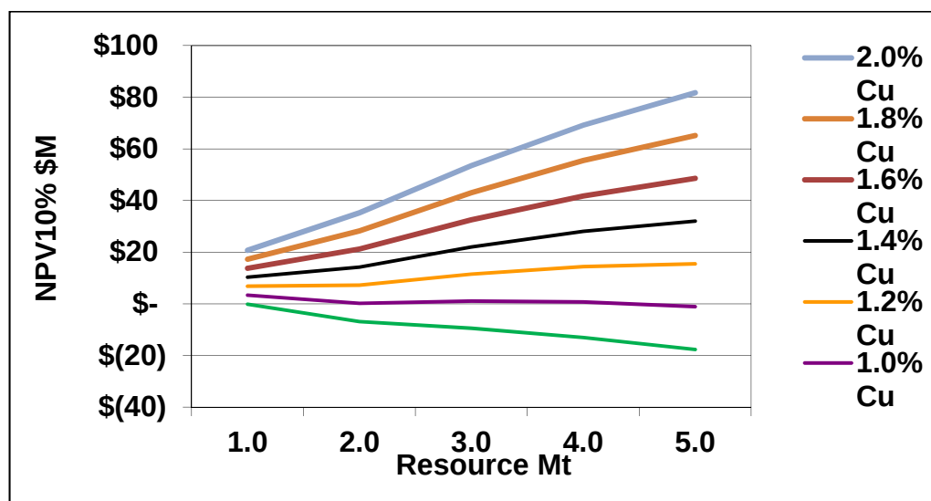
Figure 10: Impact of the additional material at various grades and tonnages from the D Zone UG
