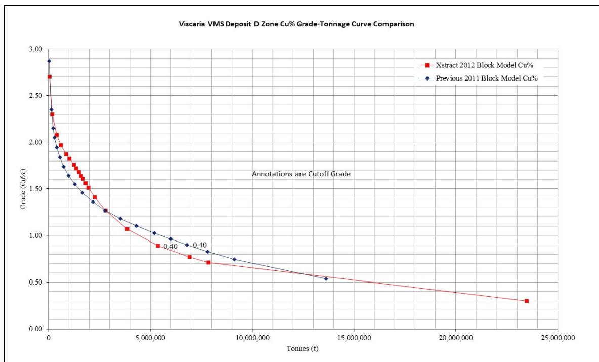
Figure 13: Grade tonnage chart for copper comparing Xstract 2012 block model vs 2011 block model
