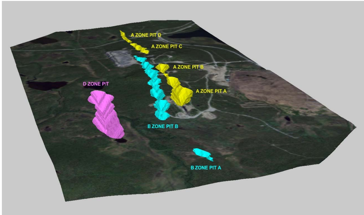
Figure 4: Site overview showing pit optimisation shells
