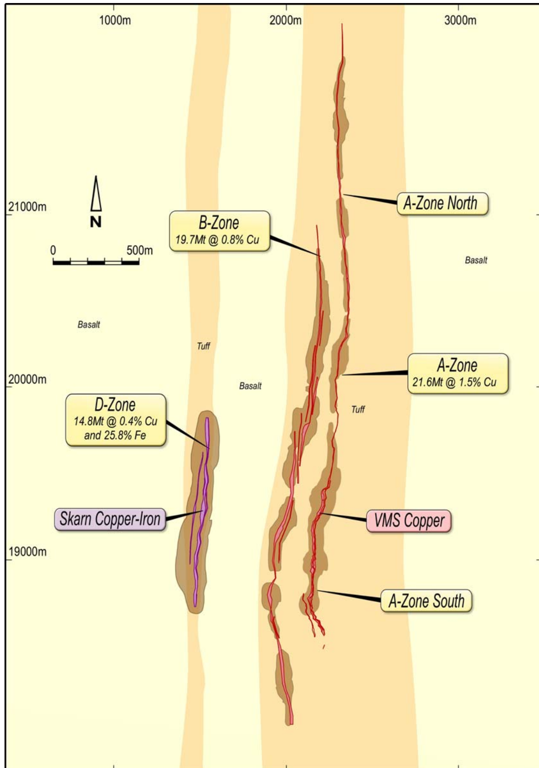
Figure 12 – Location of D Zone Mineral Resource, in relation to the A Zone and B Zone Mineral Resources (in mine grid)
