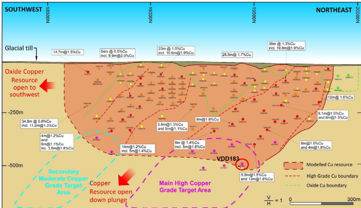
Figure 2: Schematic long section of D Zone showing current drill hole VDD183 (circled red). Other proposed holes are shown in purple.
