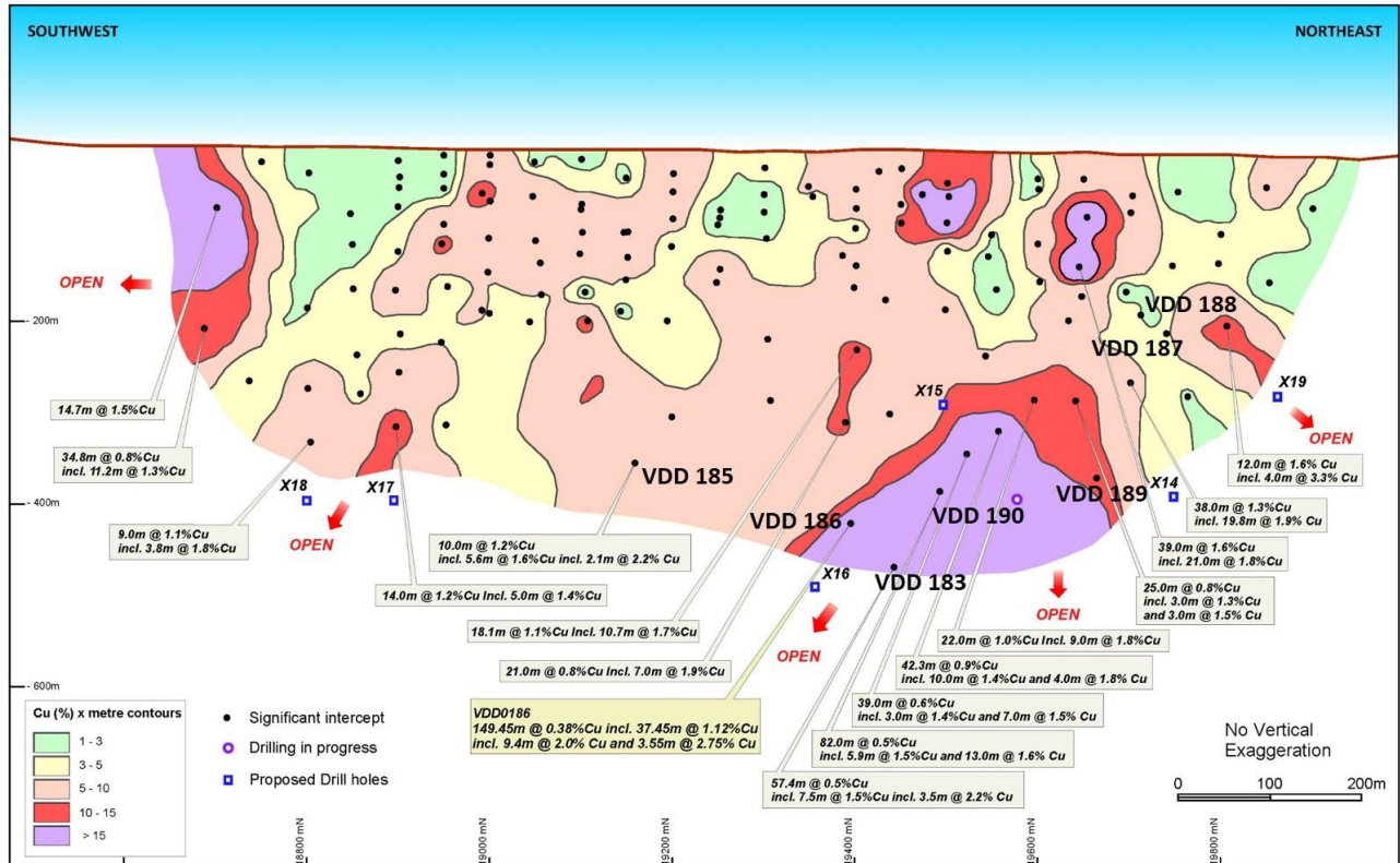
Figure 3: Location of VDD 183, 185 & 186 on schematic long section showing Cu grade x thickness contours for D Zone ironstone hosted copper mineralisation at the Viscaria Copper Project. Drill holes VDD 187-189 have been completed and assay results are pending. VDD 190 is in progress.
