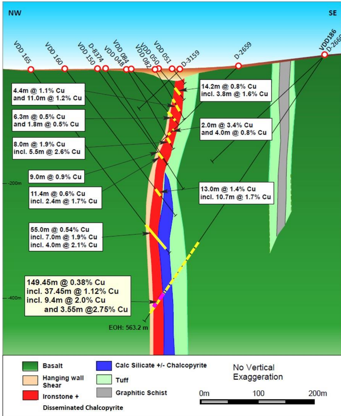
Figure 4: D Zone drill hole cross section showing results from VDD 186.
