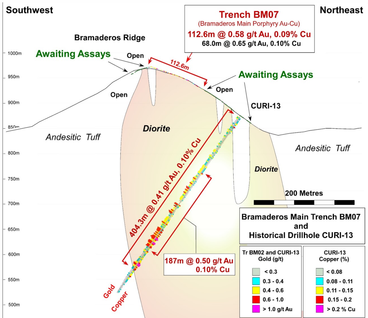
Figure 1: Cross section on Trench BM07 and historical drill hole CURI-13
