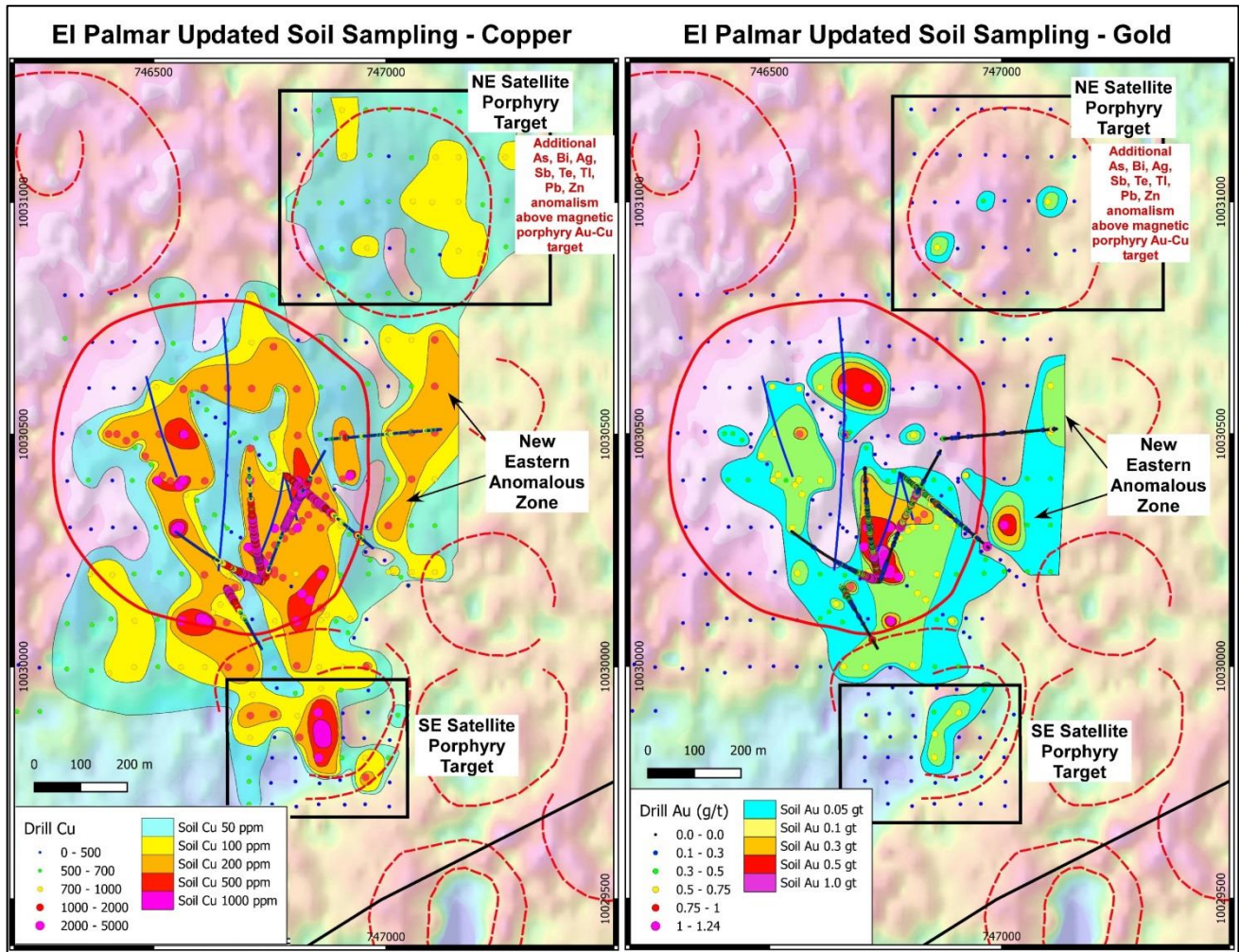
Figure 2: A composite image showing copper and gold soil anomaly over magnetics with the SE and NE satellite targets highlighted. Note also the development of an additional Eastern Anomalous Zone, which expands the size of the El Palmar target areas.
