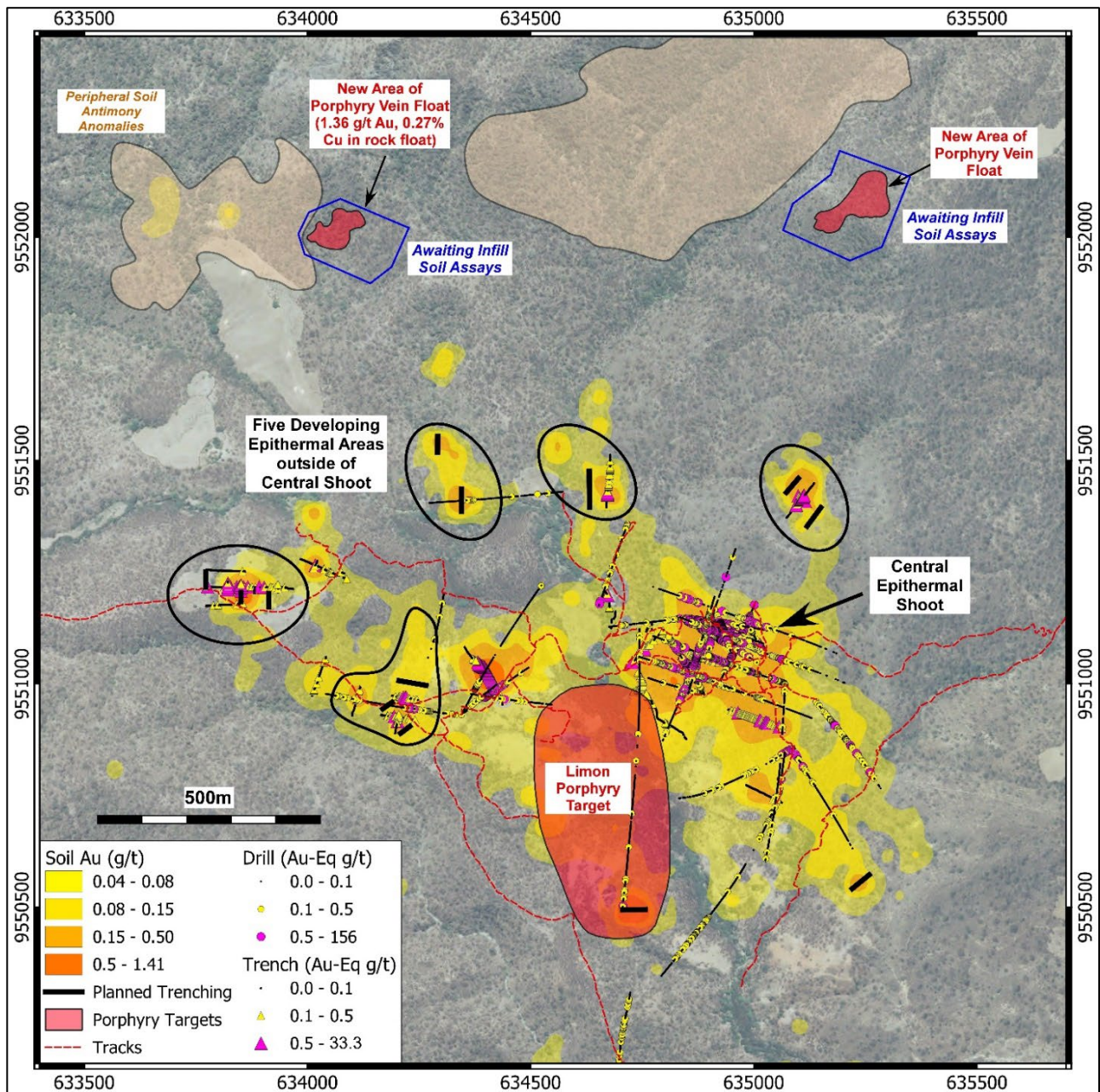
Figure 2: Broader Limon area showing new areas of porphyry gold-copper mineralisation. Limon is developing as a large 2km x 2km area of both epithermal gold-silver and porphyry gold-copper mineralisation.
