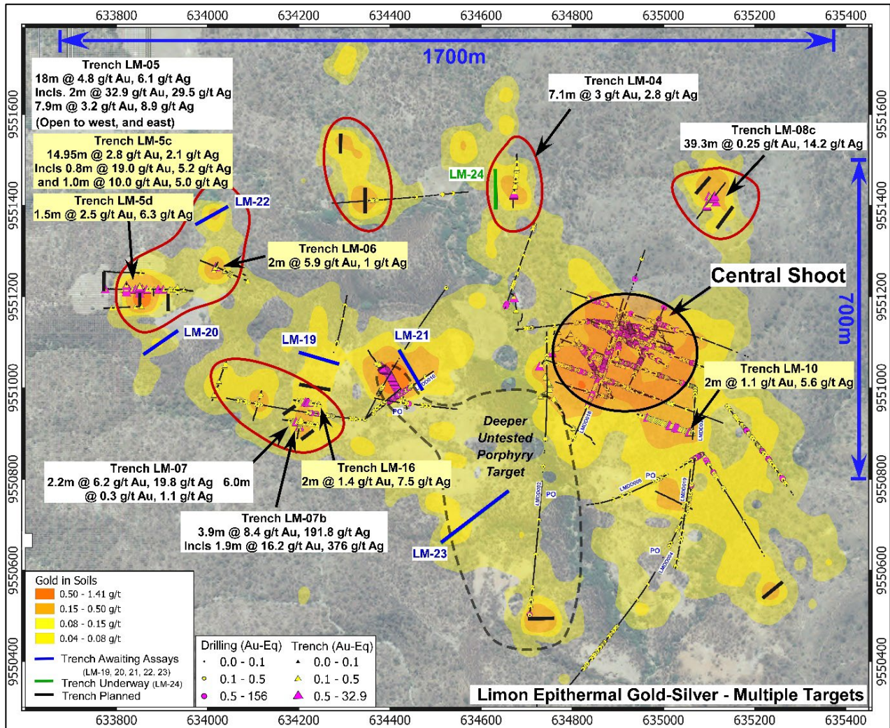
Figure 1: Limon gold-in-soils map showing extensive anomalous gold over an area of 1.7km x 700m. The circled areas have seen only partial testing. Intersections in trenches LM-5c, LM-5d, LM-10 and LM-16 from recently received assays are shown together with prior trench intersections. The black dashed line shows the Limon porphyry target outline.
