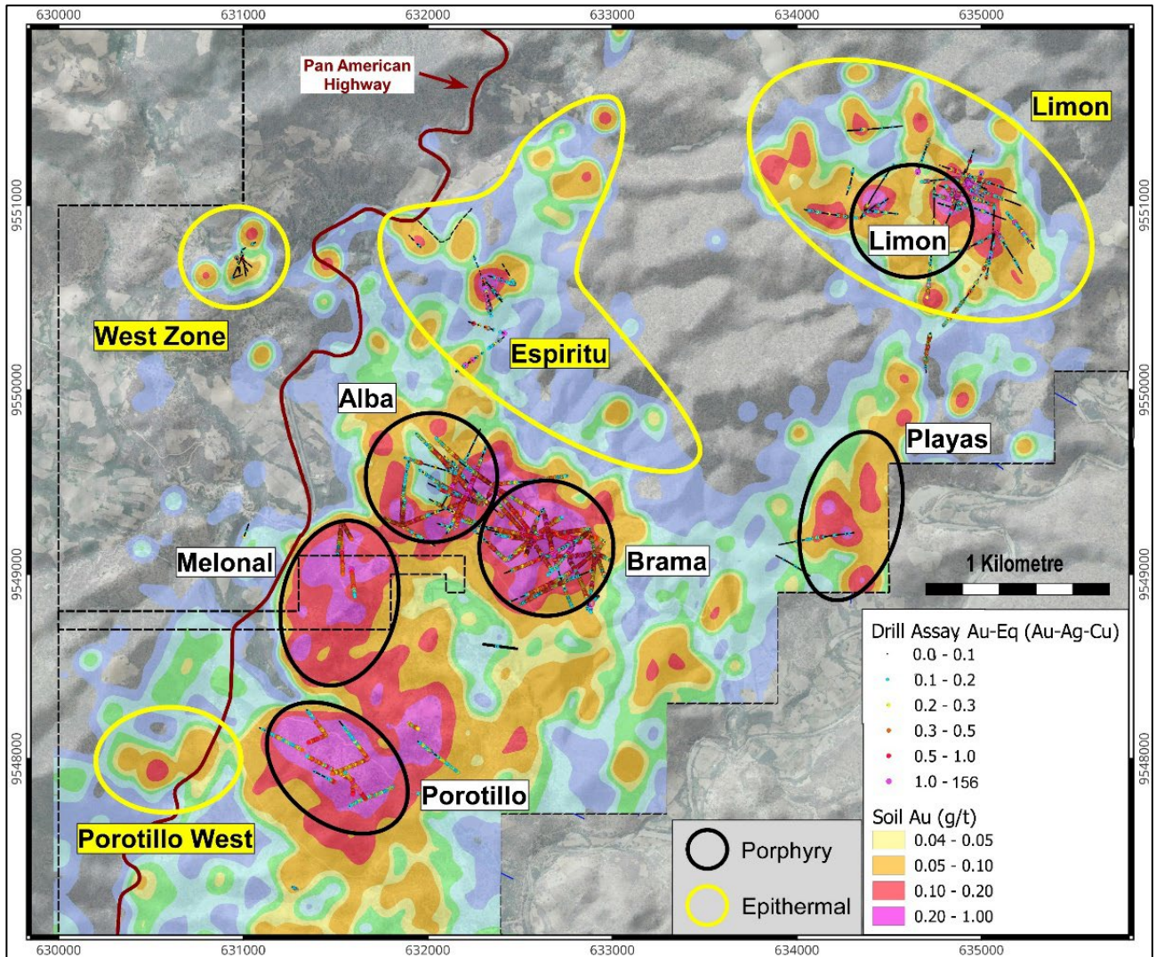
Figure 3: Gold in soil contours within the Bramaderos concession shows the main porphyry and epithermal domains.
