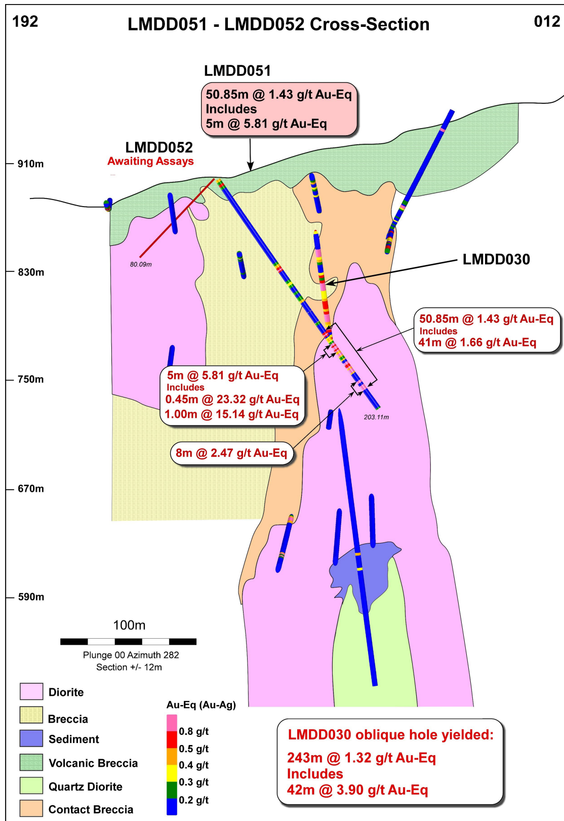
Figure 3: Cross section along drill holes LMDD051 and 052 showing mineralisation not only occurs in the surrounding breccias but also locally within a diorite body that is extensively developed at depth in the Central Shoot area. The Central shoot is plunging out of the page towards the viewer.
